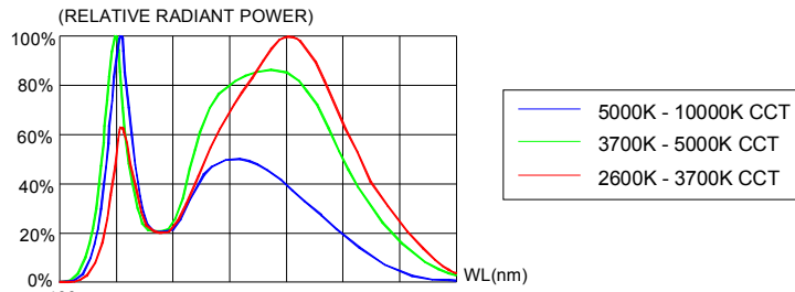
FIG.4 RELATIVE SPECTRAL POWER DISTRIBUTION
