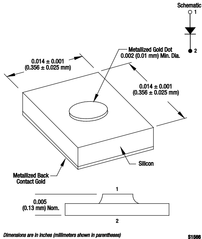
Figure 14. 150-813 Package
