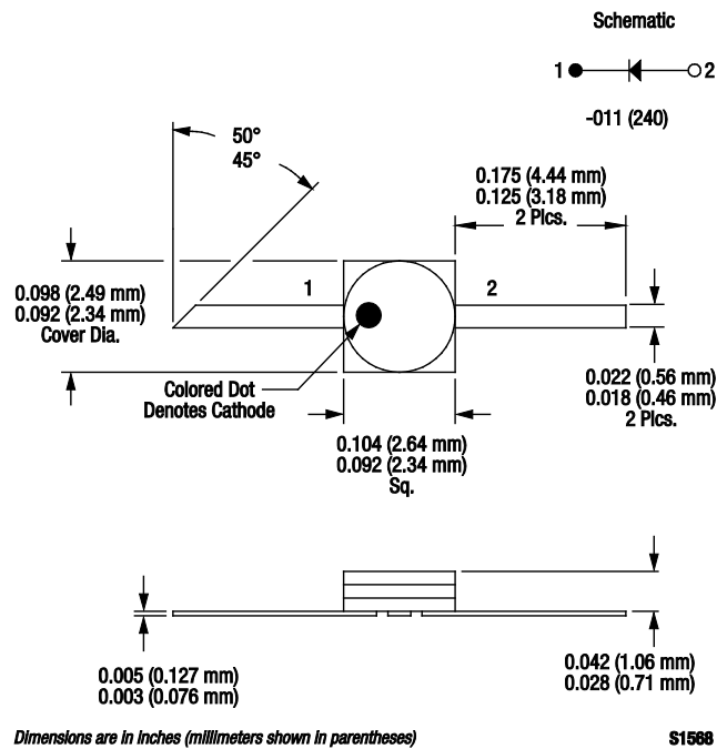
Figure 18. -240 Package
