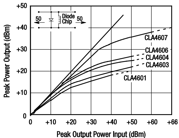
Figure 4. Typical Peak Leakage Power @ 1 GHz
