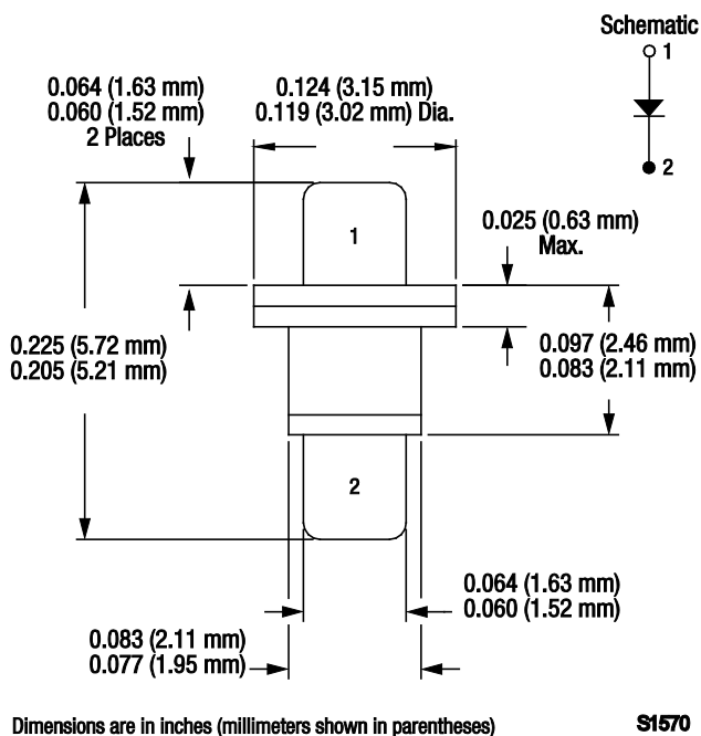
Figure 16. -210 Package
