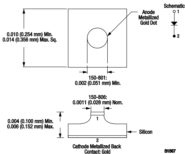
Figure 13. 150 Series Package
