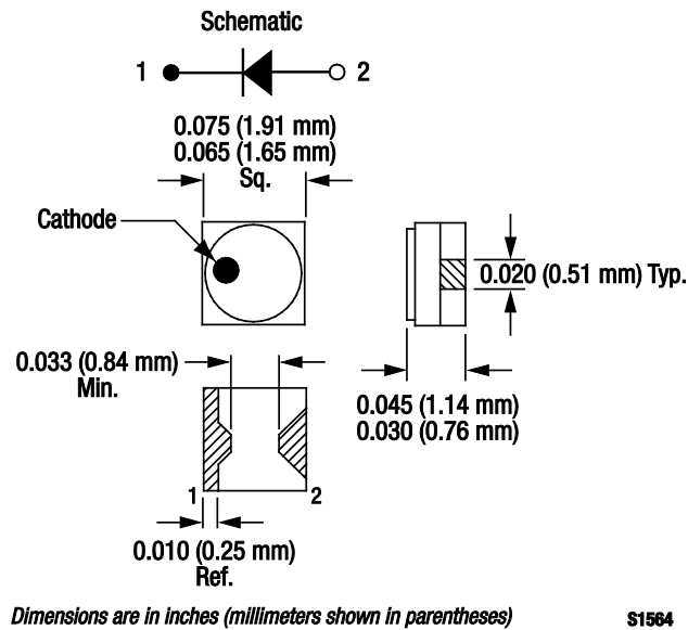
Figure 17. -219 Package
