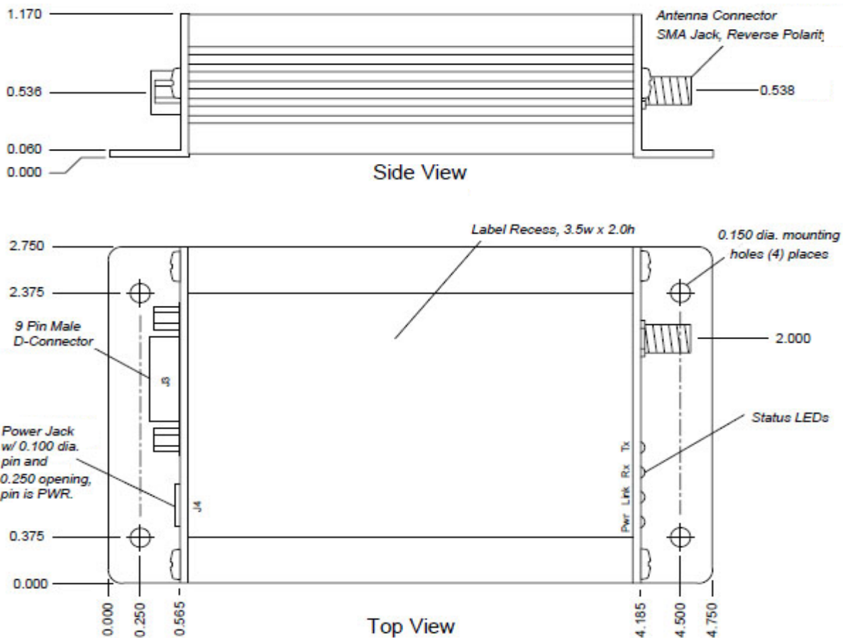
Figure 7: Mechanical Drawing
