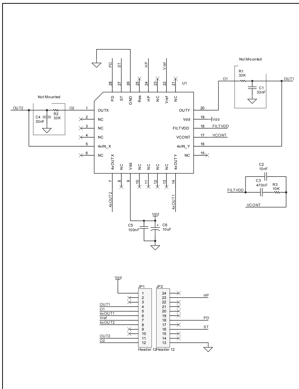
Figure 1: STEVAL-MKI099V1 circuit schematic
