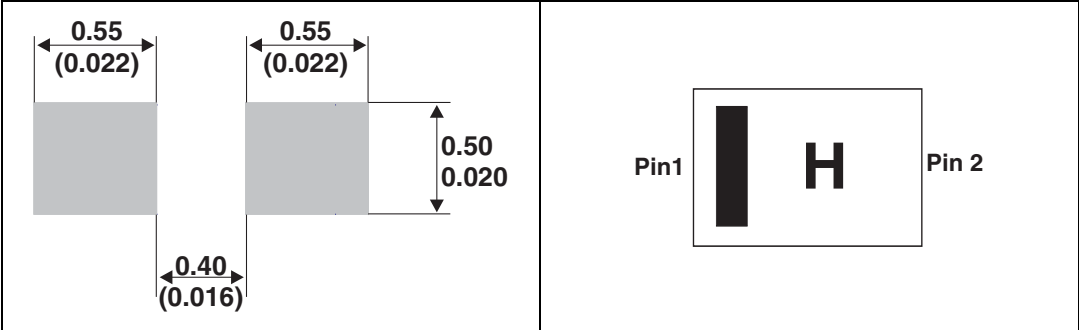
Figure 20. SOD882T footprint in mm (inches)
