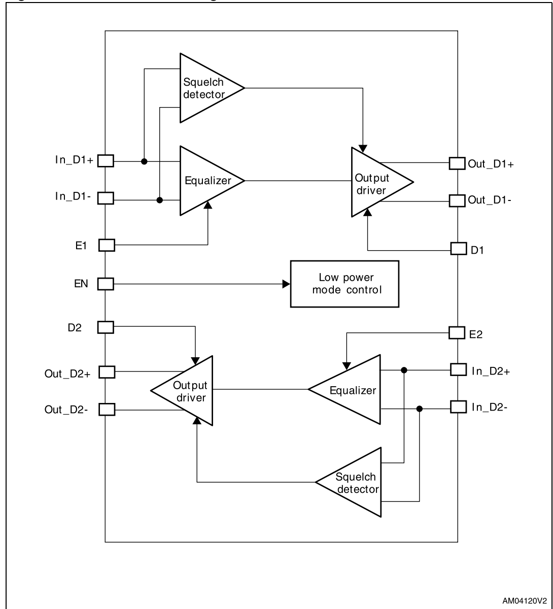
Figure 1. STA1102R block diagram
