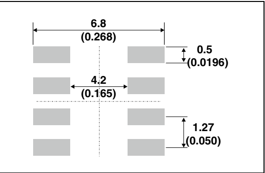
Figure 15. Footprint recommendation for improved clearance dimensions in mm (inches)
