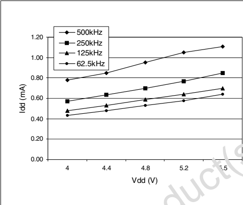
Figure 65. Typical I_{DD} in Slow mode
