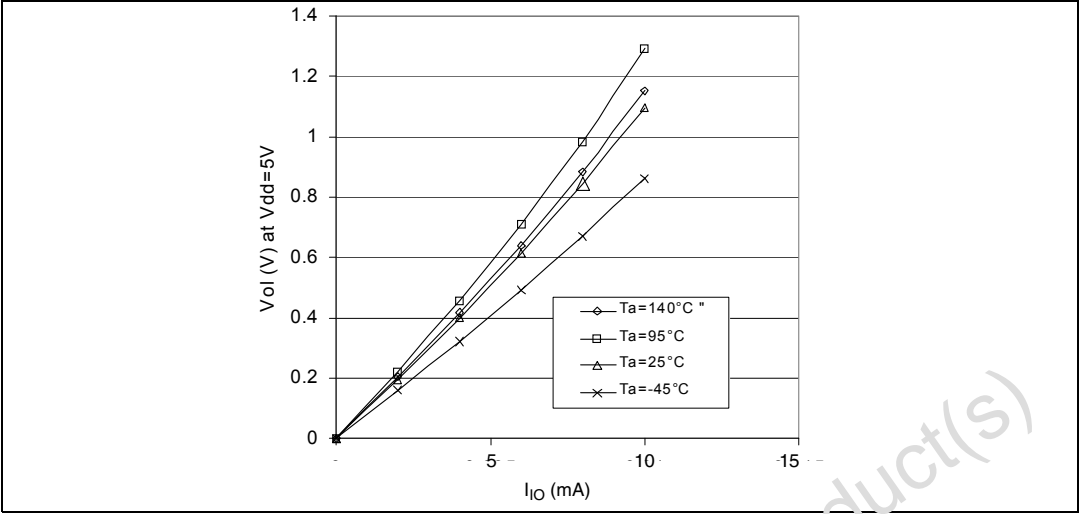
Figure 73. Typical V_{OL} at V_{DD} = 5V (standard ports)
