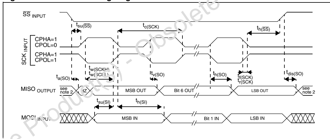
Figure 83. SPI slave timing diagram with CPHA = 1 (1)
