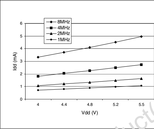
Figure 66. Typ. I_{DD} in Slow Wait mode
