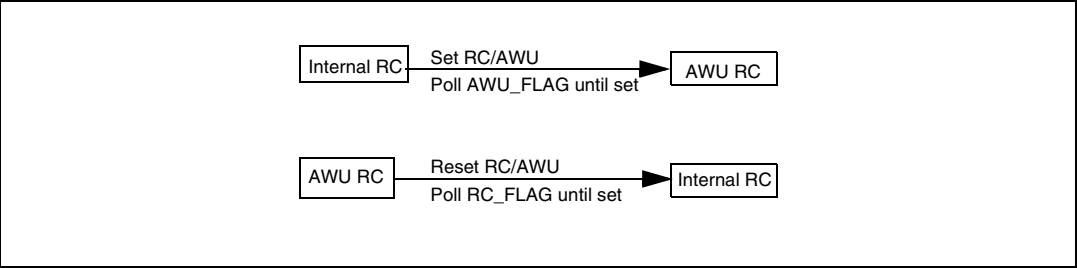
Figure 13. Clock switching
