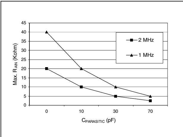
Figure 94. R_{AIN} maximum versus f_{ADC} with C_{AIN} = 0\text{pF}^{(1)}
