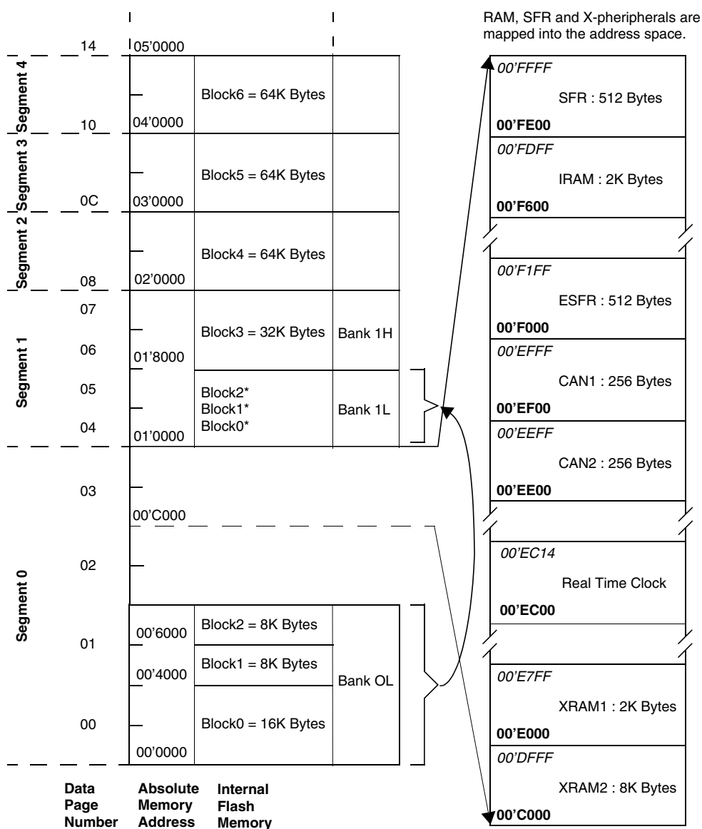
Figure 4 : ST10F269-T3 On-chip Memory Mapping
