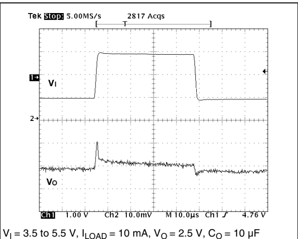
Figure 16. Line transient
