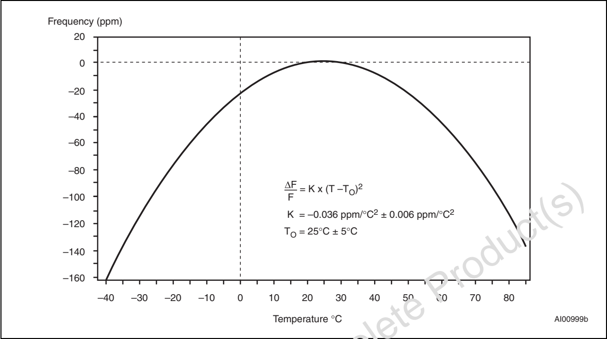
Figure 12. Crystal accuracy across temperature
