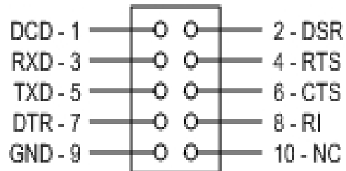
10 Pin Header Pin Out Top View
