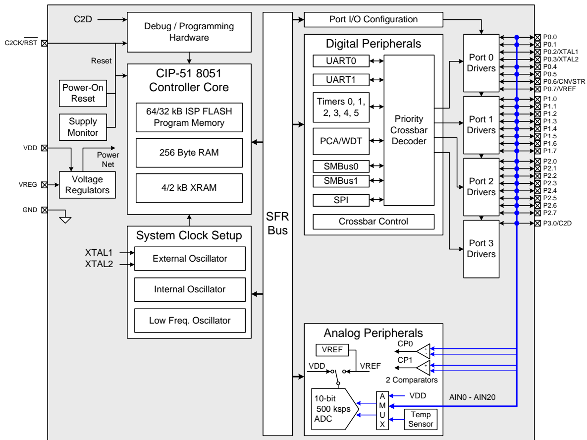
Figure 1.2. C8051F389/B Block Diagram
