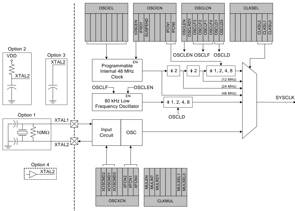
Figure 19.1. Oscillator Options
