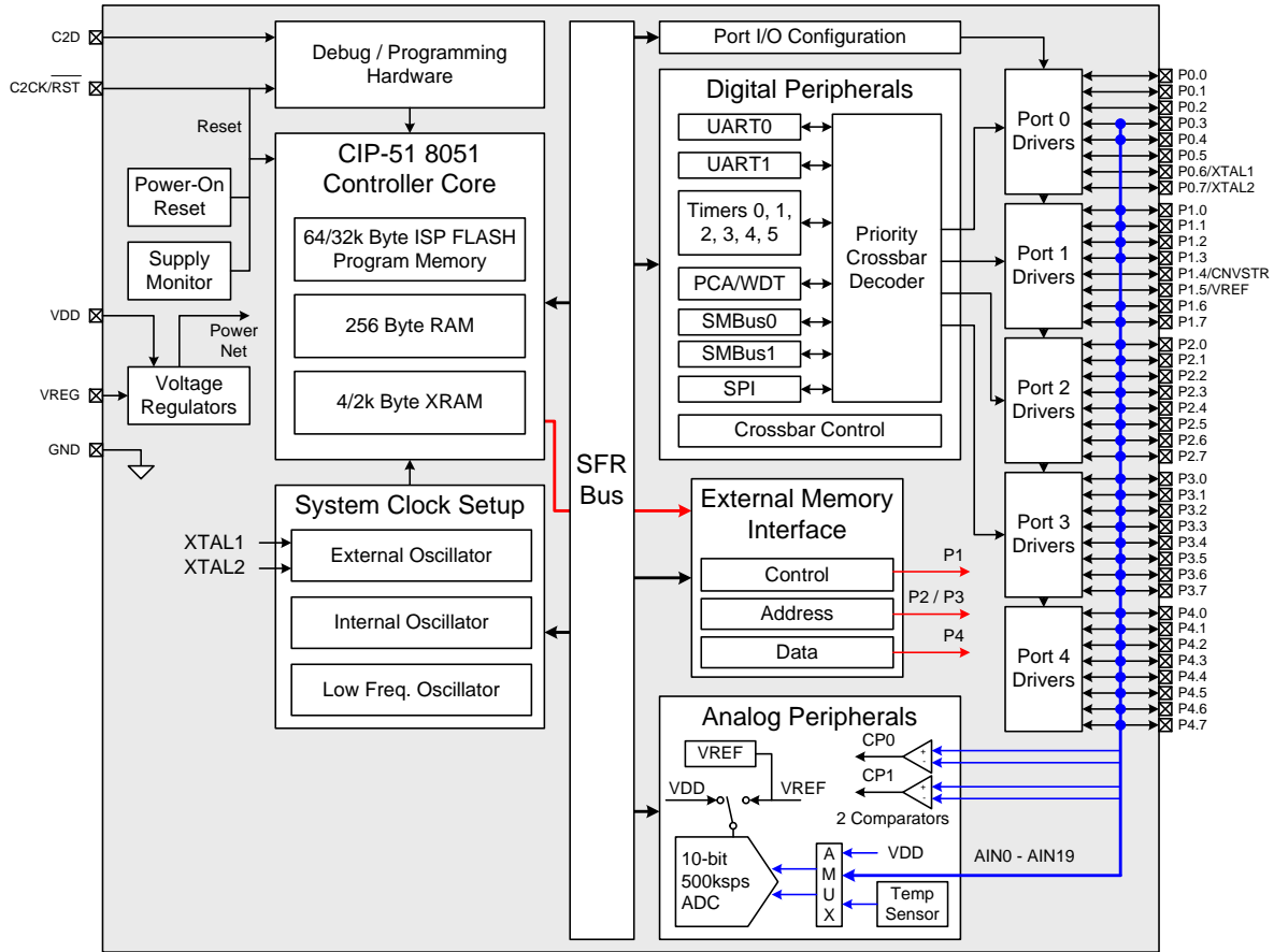
Figure 1.1. C8051F388/A Block Diagram
