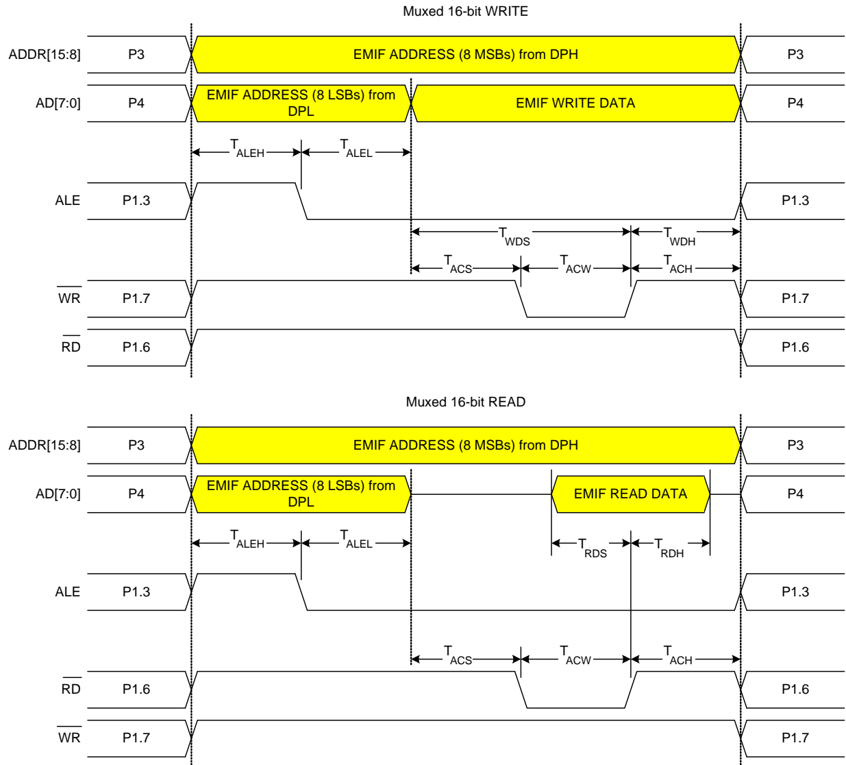
Figure 14.7. Multiplexed 16-bit MOVX Timing
