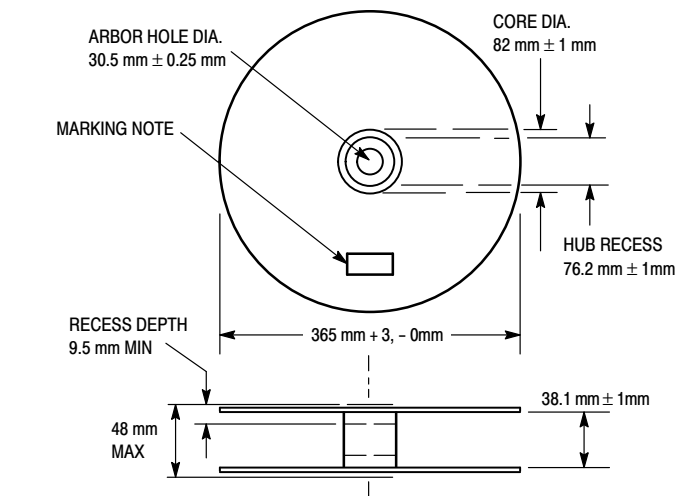
Figure 51. Reel Specifications
