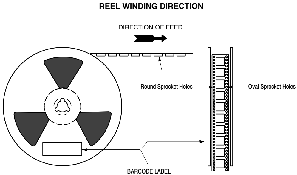
Figure 42. Round and Oval Sprocket Holes Used with 32 mm, 42 mm, 44 mm and 52 mm Tape (holes on both sides)
