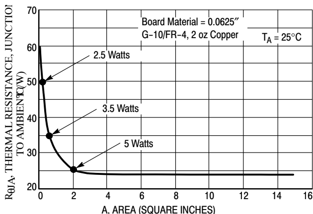
Figure 59. Thermal Resistance versus Drain Pad Area for the D²PAK Package (Typical)
