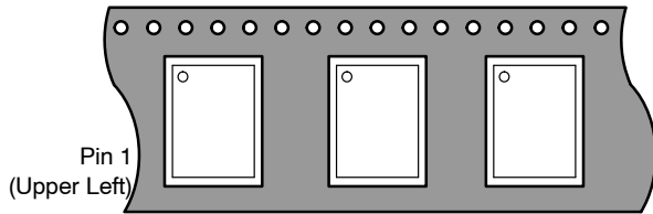
Figure 37. DFN/QFN/WLCSP-5
