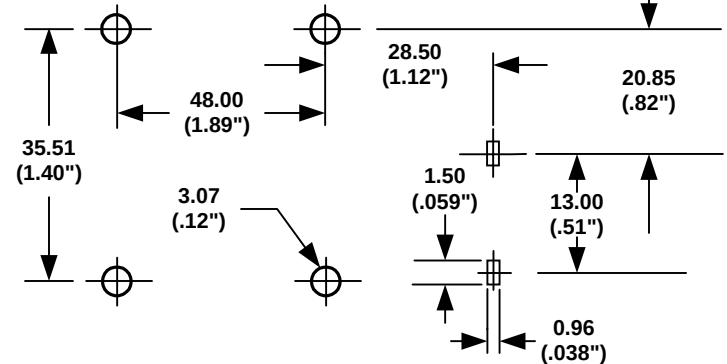
PCB LAYOUT
