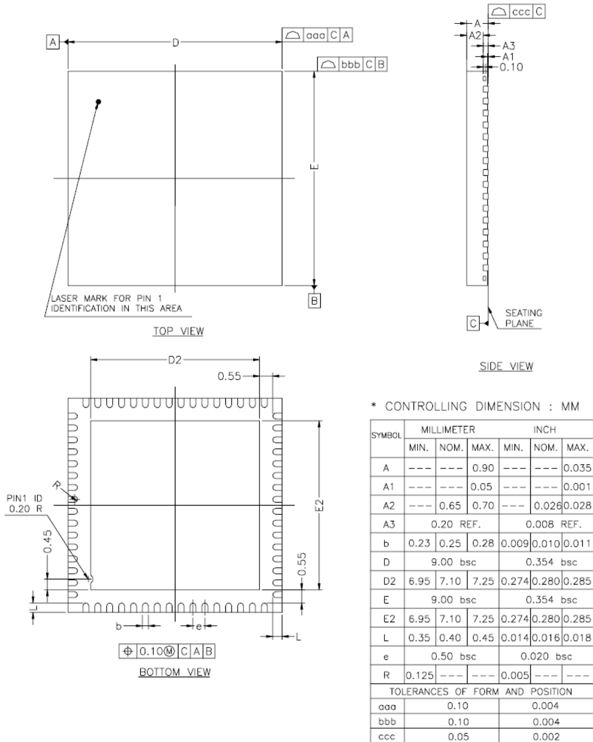
Figure 5-5. 64-lead QFN Package Mechanical Drawing
