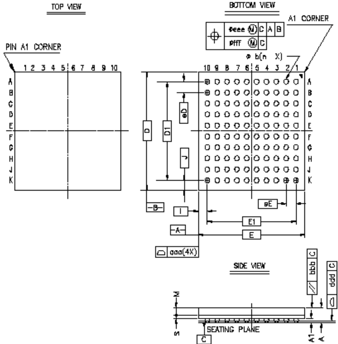
Figure 5-3. 100-ball VFBGA Package Mechanical Drawing
