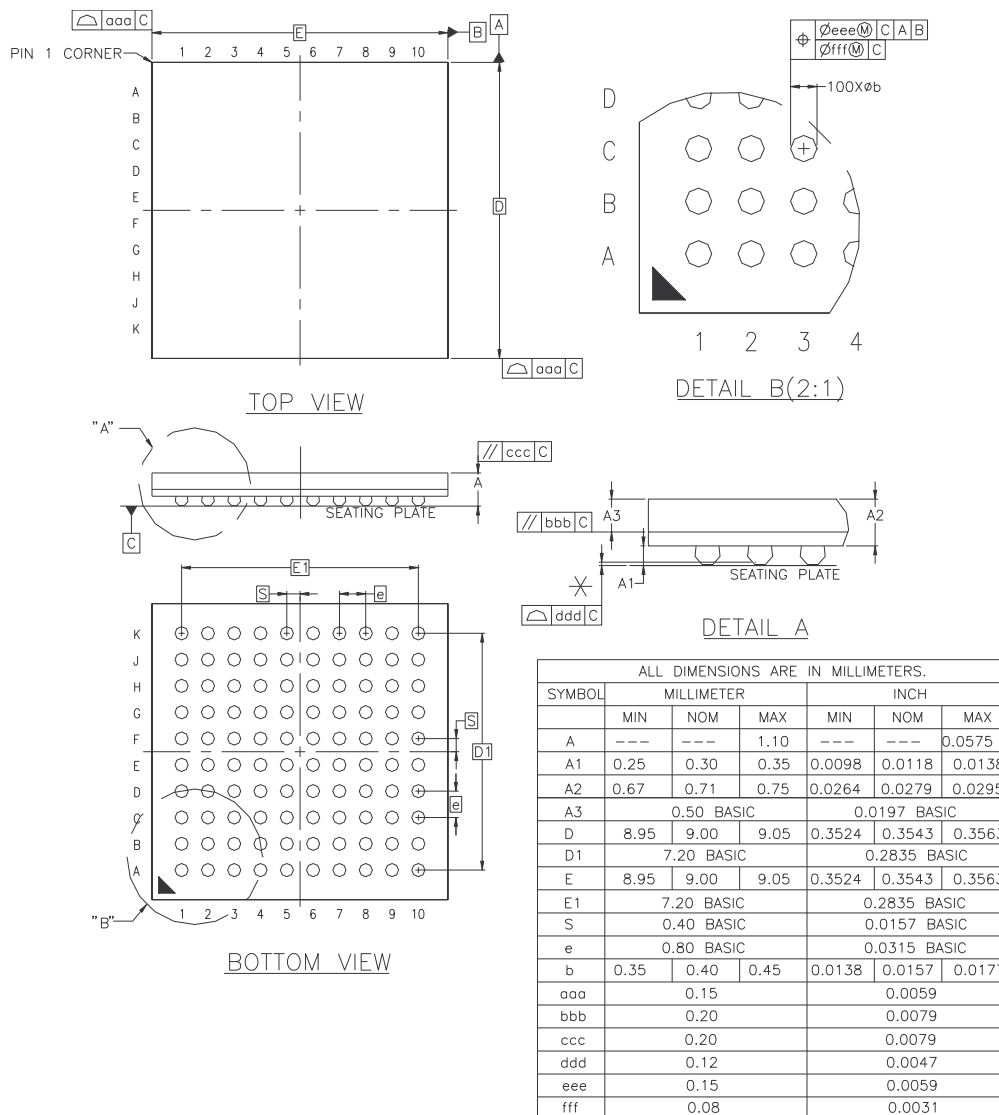
Figure 5-2. 100-ball TFBGA Package Mechanical Drawing
