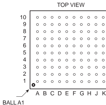
Figure 4-2. Orientation of the 100-ball TFBGA Package
