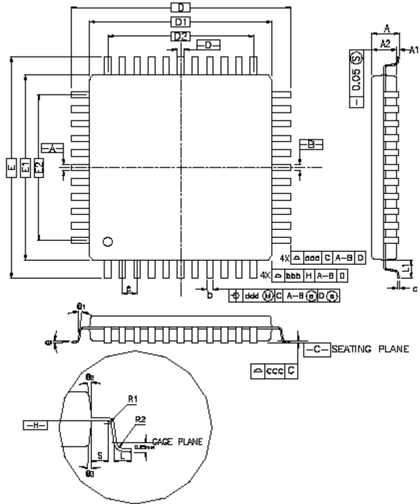
Figure 5-4. 64-lead LQFP Package Mechanical Drawing
