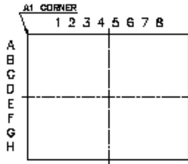
Figure 4-6. Orientation of the 64-ball WLCSP Package
