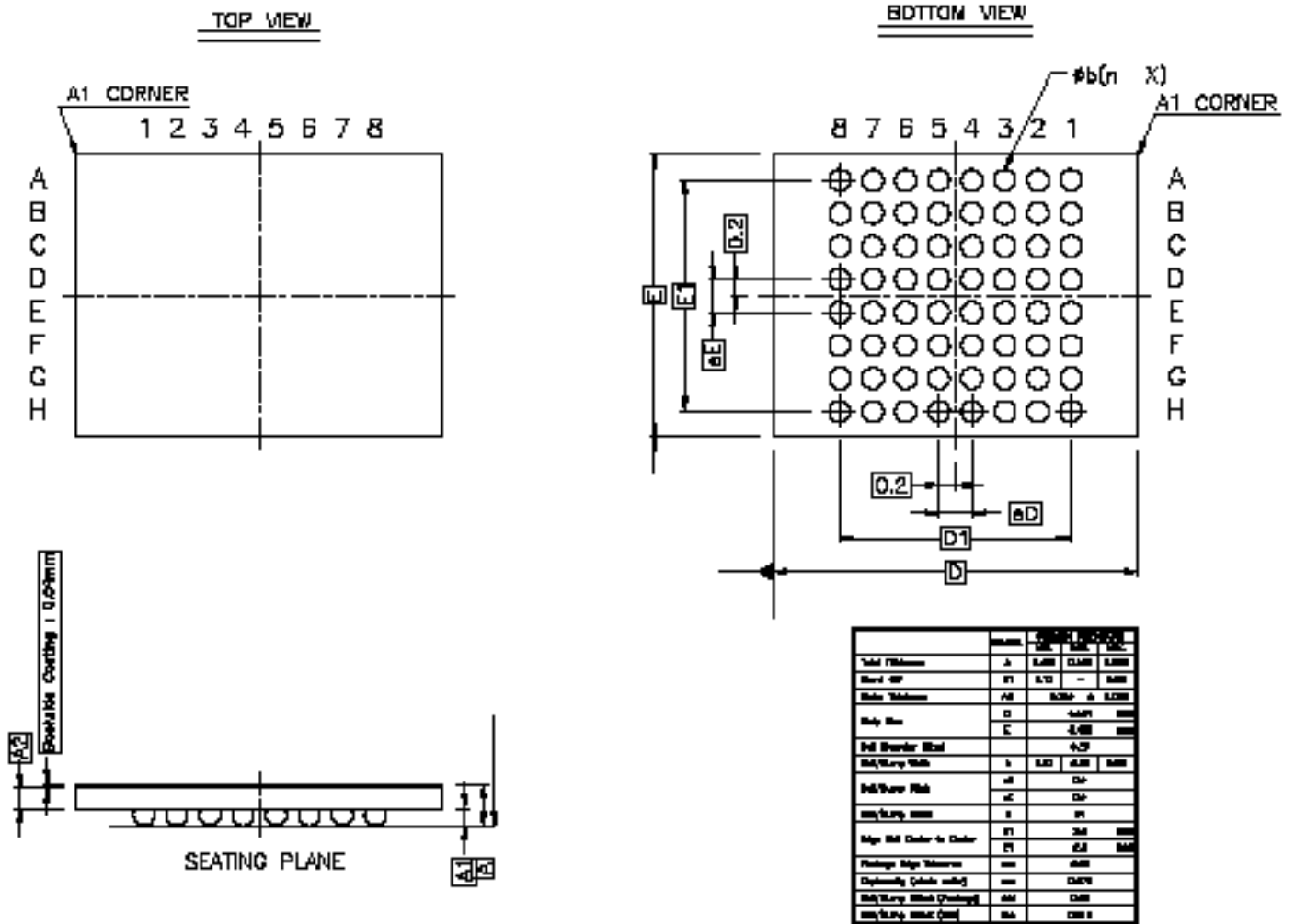
Figure 5-6. 64-ball WLCSP Package Mechanical Drawing
