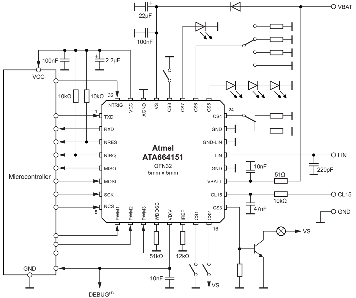
Figure 16-2. Application Example 1: LIN Slave with Different External Circuitry at the CSx-pins
