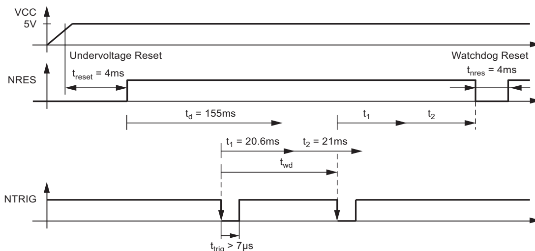
Figure 10-1. Timing Sequence with R_{\text{WD\_osc}} = 51\text{k}\Omega
