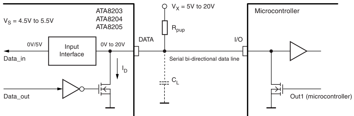
Figure 13-2. Data Interface
