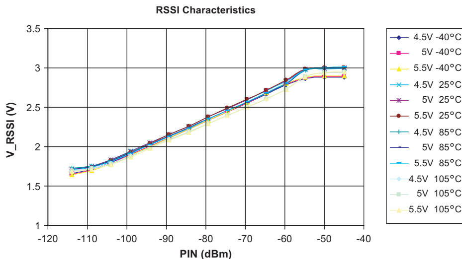
Figure 4-1. RSSI Characteristics ATA5724
