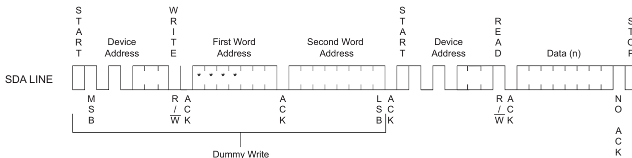
Figure 10-2. Random Read
