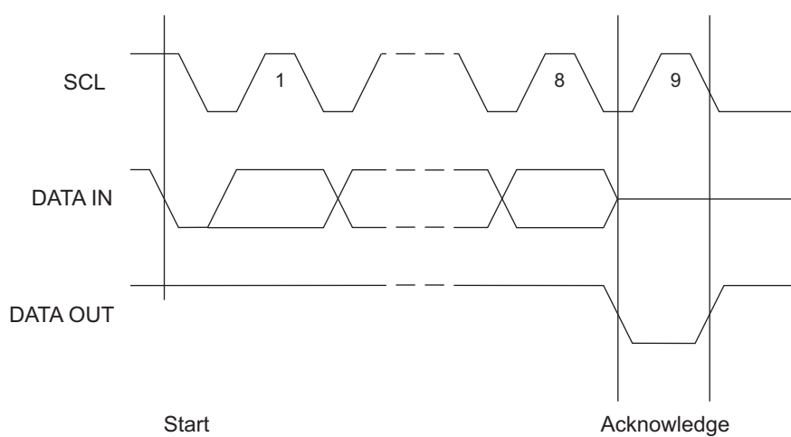
Figure 7-6. Output Acknowledge
