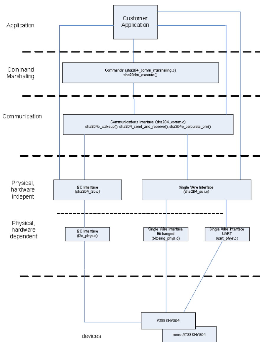
Figure 1. ATECC108/ATSHA204 Firmware Library Design
