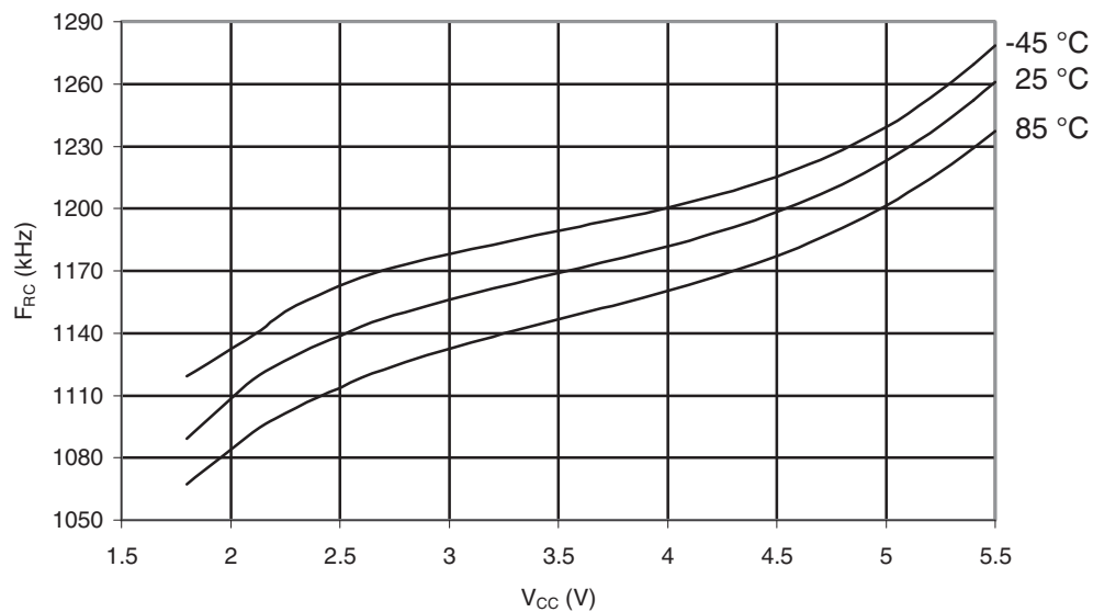
Figure 30-410. ATmega645A: Watchdog Oscillator Frequency vs. V_{CC}
