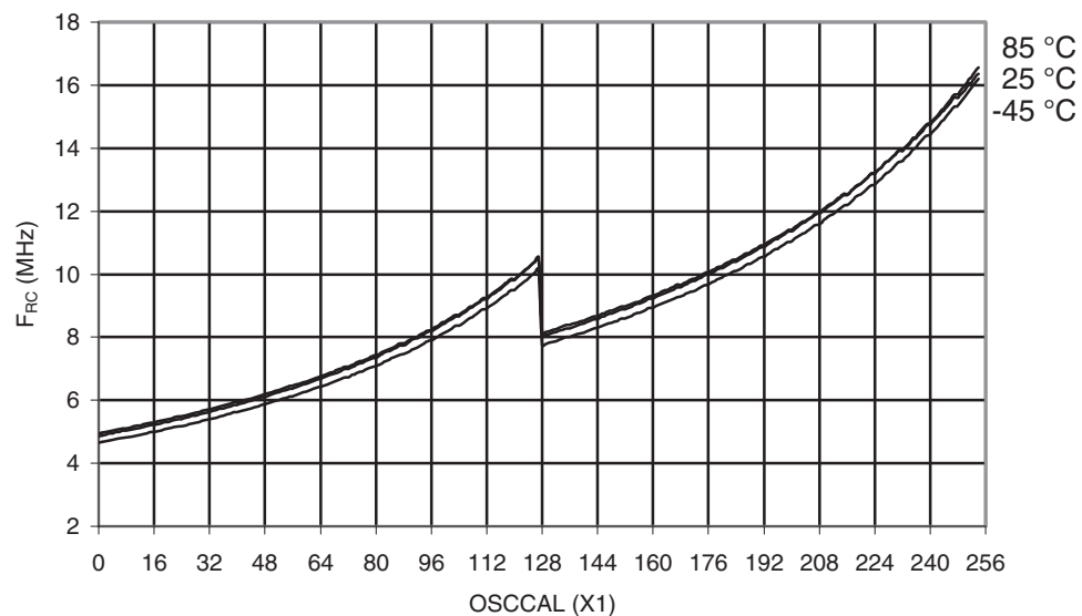
Figure 30-597. ATmega6450P: Calibrated 8MHz RC Oscillator Frequency vs. Oscal Value
