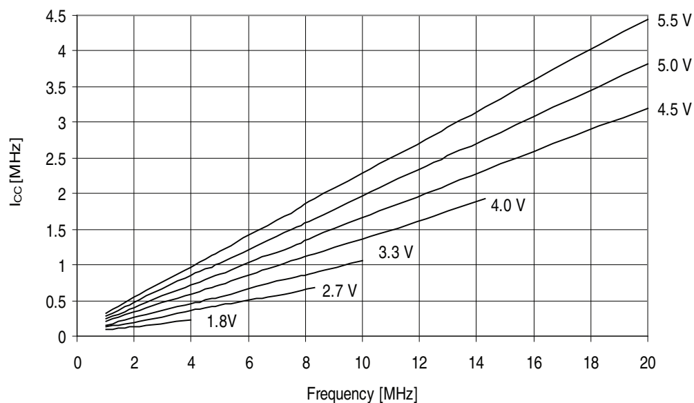
Figure 31-246. ATmega3250A: Idle Supply Current vs. Frequency (1 - 20MHz)
