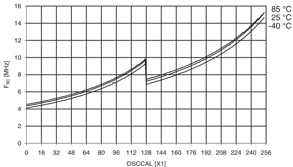
Figure 30-353. ATmega3250PA: Calibrated 8MHz RC Oscillator Frequency vs. Oscal Value
