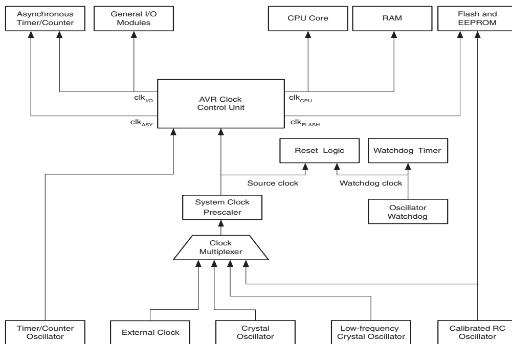
Figure 9-1. Clock distribution.
