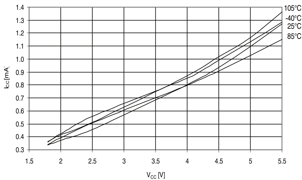
Figure 31-243. ATmega3250A: Active Supply Current vs. V_{CC} (Internal RC Oscillator, 1 MHz)
