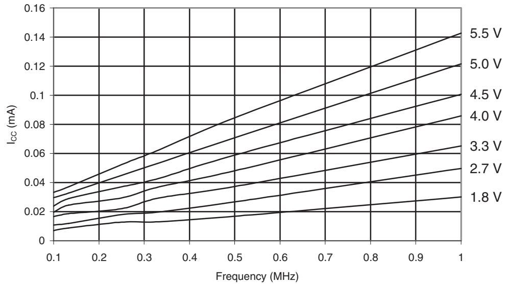
Figure 30-484. ATmega645P: Reset Supply Current vs. V_{CC} (0.1 - 1.0MHz, Excluding Current Through The Reset Pull-up)
