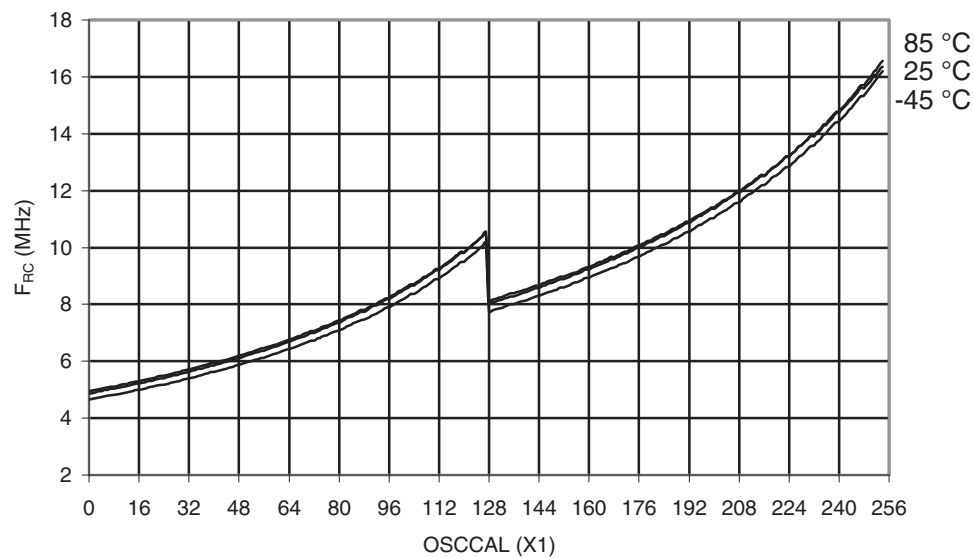
Figure 30-536. ATmega6450A: Calibrated 8MHz RC Oscillator Frequency vs. Oscal Value
