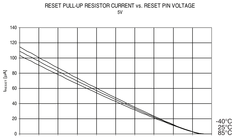
Figure 30-203. ATmega325PA: Reset Pull-up Resistor Current vs. Reset Pin Voltage ( V_{CC} = 5V )
