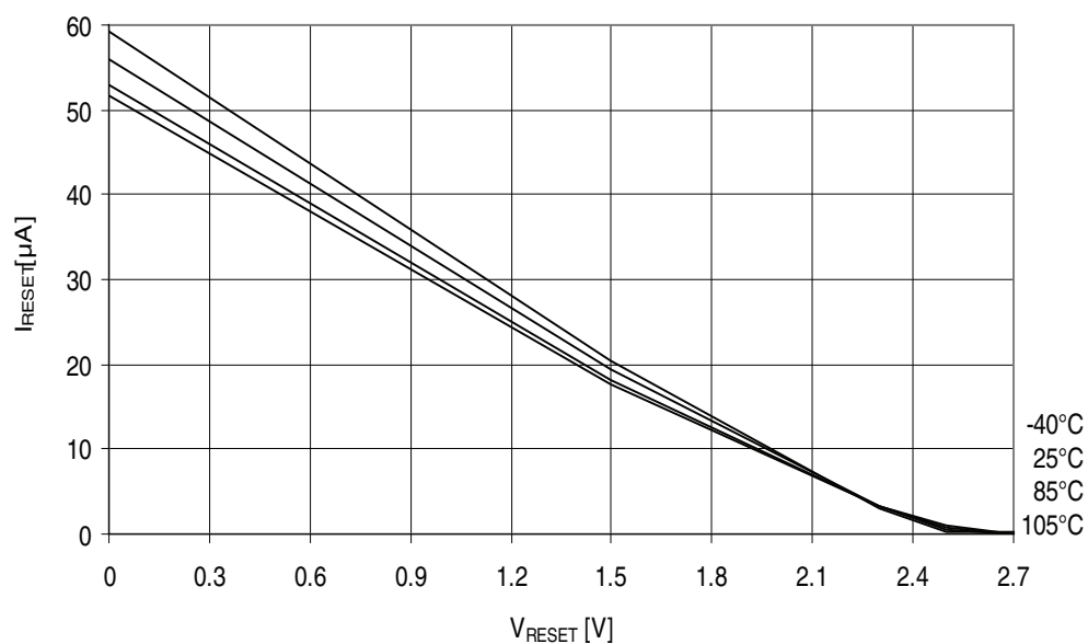
Figure 31-323. ATmega3250PA: Reset Pull-up Resistor Current vs. Reset Pin Voltage ( V_{CC} = 2.7V )
