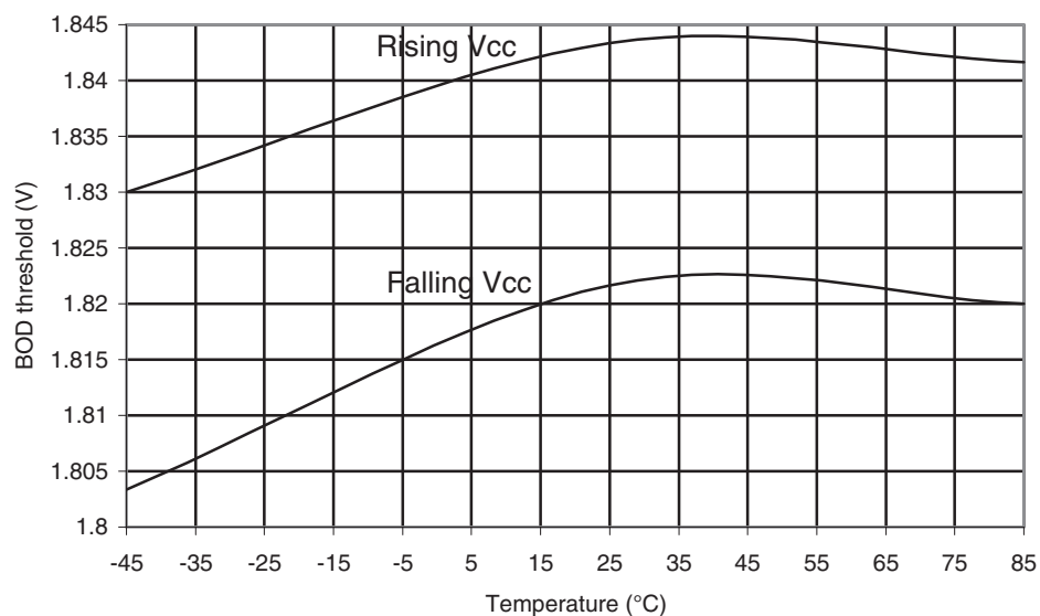
Figure 30-468. ATmega645P: BOD Thresholds vs. Temperature (BOD Level is 1.8V)
