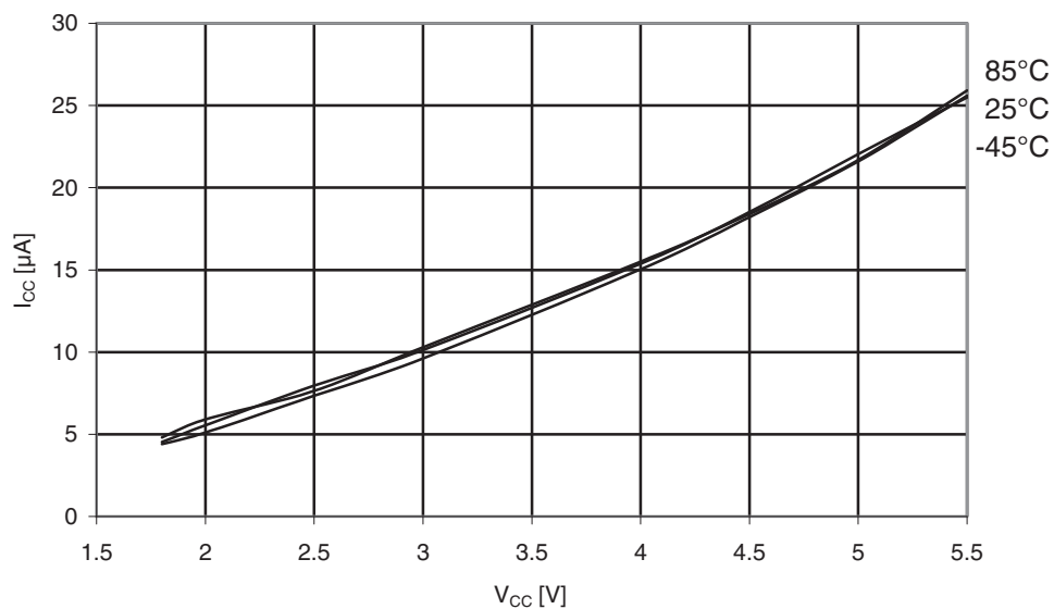
Figure 30-58. ATmega165A: Analog Comparator current vs. V_{CC} .
