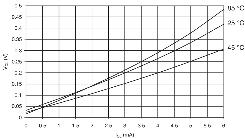
Figure 30-459. ATmega645P: I/O Pin Output Voltage vs. Sink Current, Port B ( V_{CC} = 1.8V )
