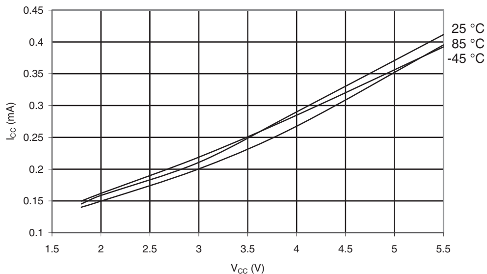
Figure 30-373. ATmega645A: Idle Supply Current vs. V_{CC} (Internal RC Oscillator, 1MHz)
