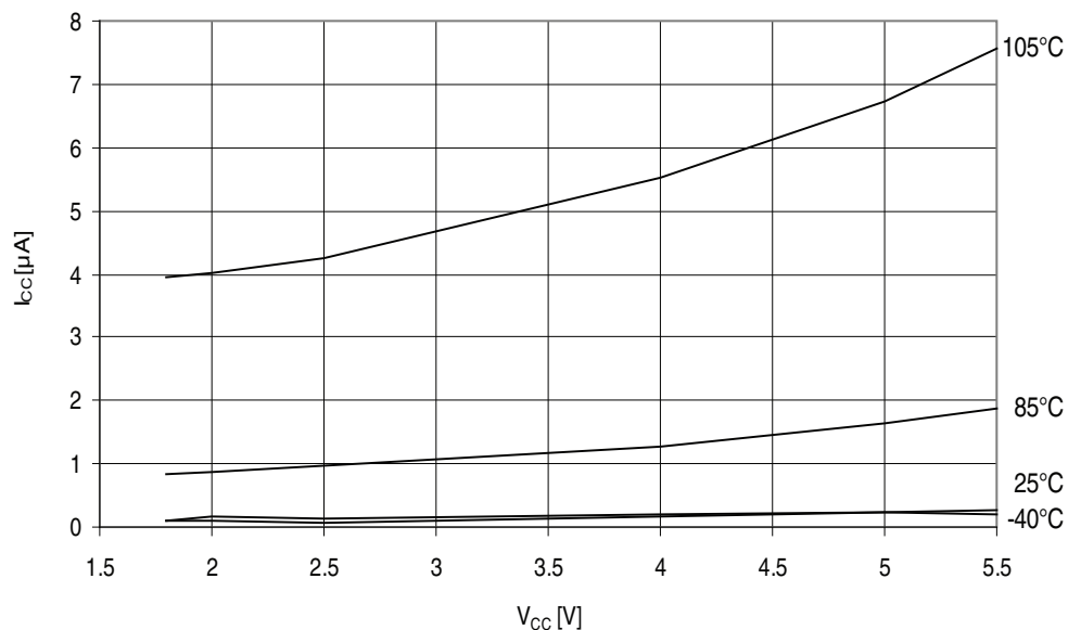
Figure 31-134. ATmega325PA: Power-down Supply Current vs. V_{CC} (Watchdog Timer Disabled)
