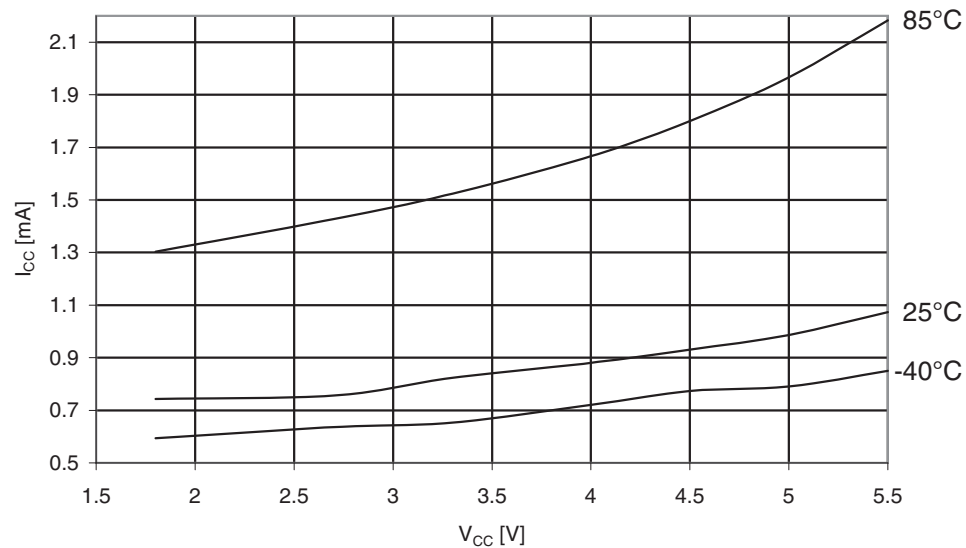
Figure 30-198. ATmega325PA: Standby Supply Current vs. V_{CC} (32kHz Watch XTAL, Watchdog Timer Disabled)
