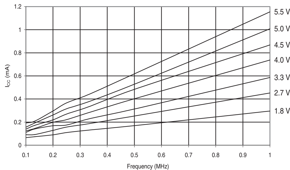
Figure 30-548.ATmega6450A: Active Supply Current vs. Low Frequency (0.1 - 1.0MHz)
