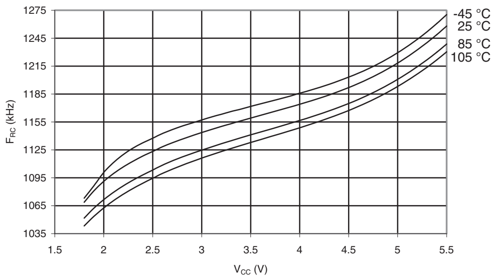
Figure 31-45. ATmega165PA: Watchdog Oscillator Frequency vs. V_{CC}
