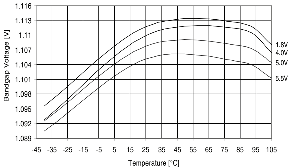
Figure 31-283. ATmega325A: Bandgap Voltage vs. Temperature
