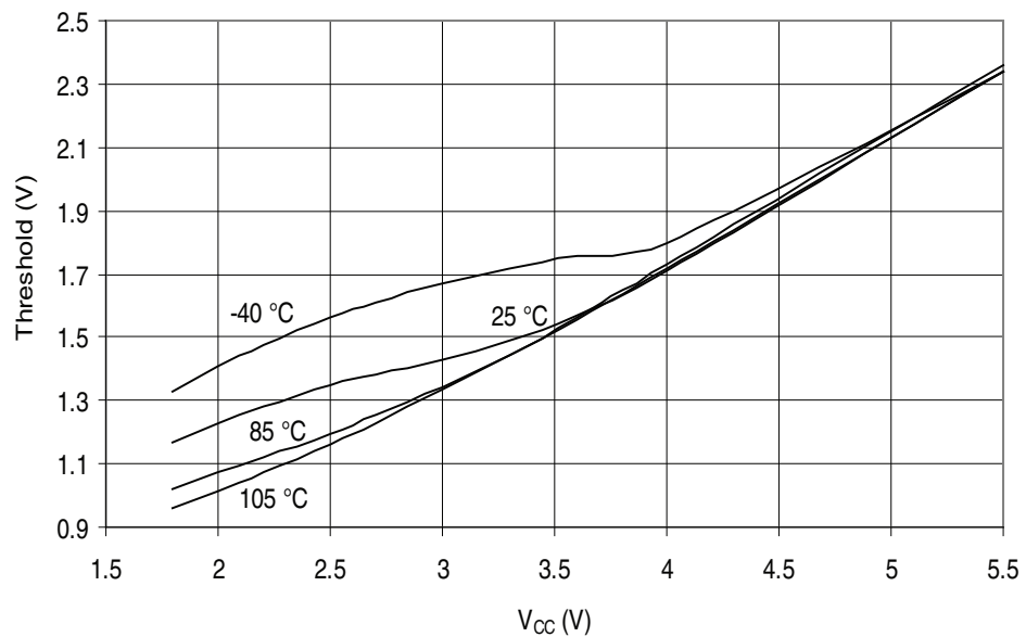
Figure 31-276. ATmega3250A: Reset Input Threshold Voltage vs. V_{CC} ( V_{IH} , Reset Pin Read as “1”)
