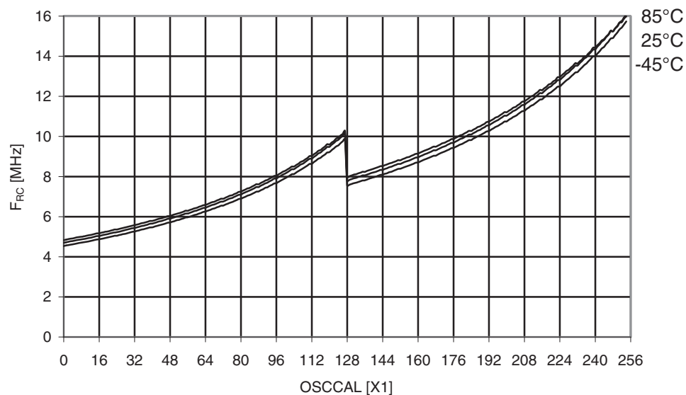
Figure 30-51. Atmel ATmega165A: Calibrated 8MHz RC oscillator frequency vs. Osccal value.
