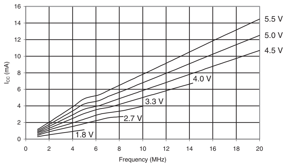
Figure 30-366. ATmega645A: Active Supply Current vs. Frequency (1 - 20MHz)
