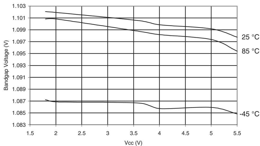
Figure 30-469. ATmega645P: Bandgap Voltage vs. V_{CC}
