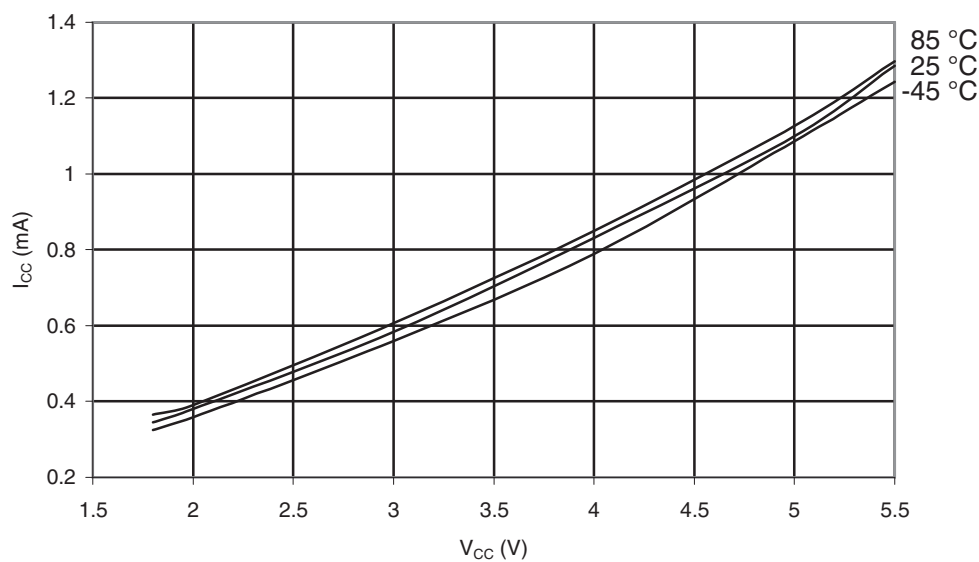
Figure 30-368. ATmega645A: Active Supply Current vs. V_{CC} (Internal RC Oscillator, 1MHz)
