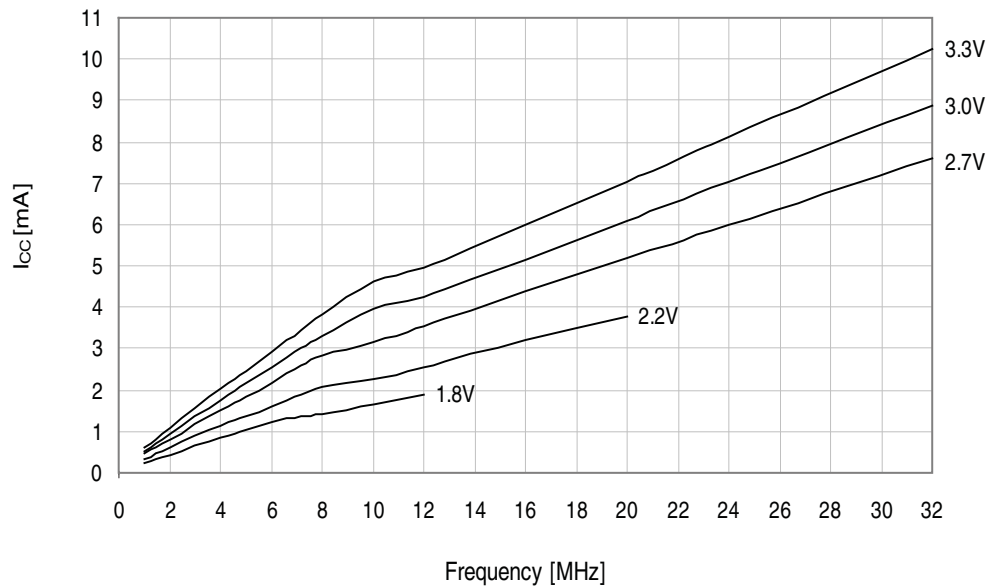
Figure 33-220. Active supply current vs. frequency. f_{\text{SYS}} = 1 - 32\text{MHz} external clock, T = 25^\circ\text{C} .
