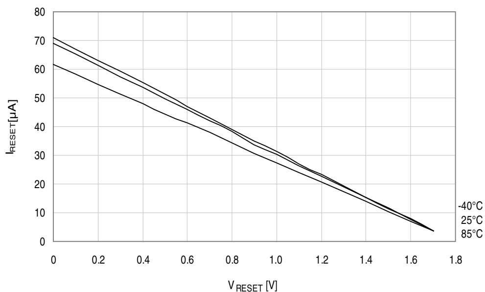
Figure 33-334. Reset pin pull-up resistor current vs. reset pin voltage. V_{CC} = 1.8V .
