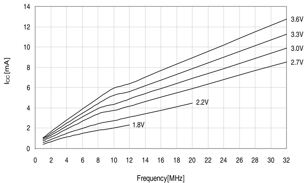
Figure 33-287. Active supply current vs. frequency. f_{\text{SYS}} = 1 - 32\text{MHz} external clock, T = 25^\circ\text{C} .
