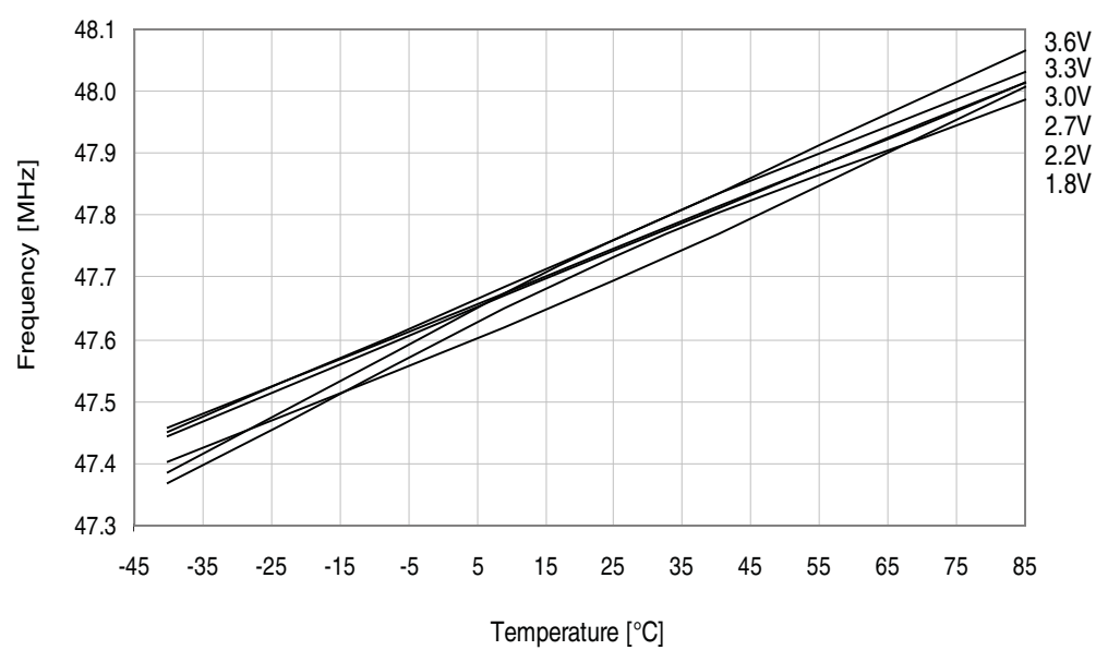
Figure 33-282. 48MHz internal oscillator frequency vs. temperature. DFLL enabled, from the 32.768kHz internal oscillator.
