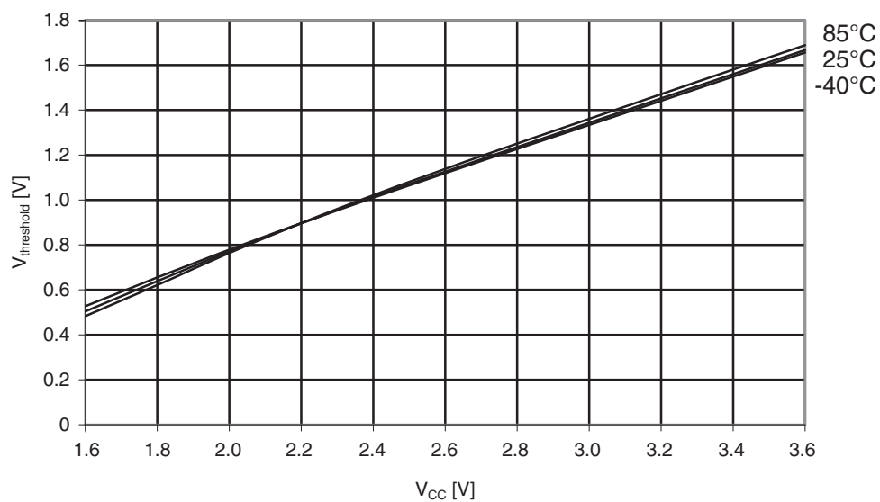
Figure 33-28. I/O pin input threshold voltage vs. V_{CC} .
