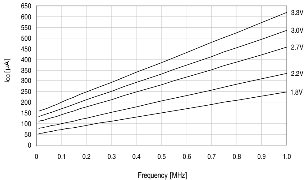
Figure 33-219. Active supply current vs. frequency. f_{\text{SYS}} = 0 - 1\text{MHz} external clock, T = 25^\circ\text{C} .
