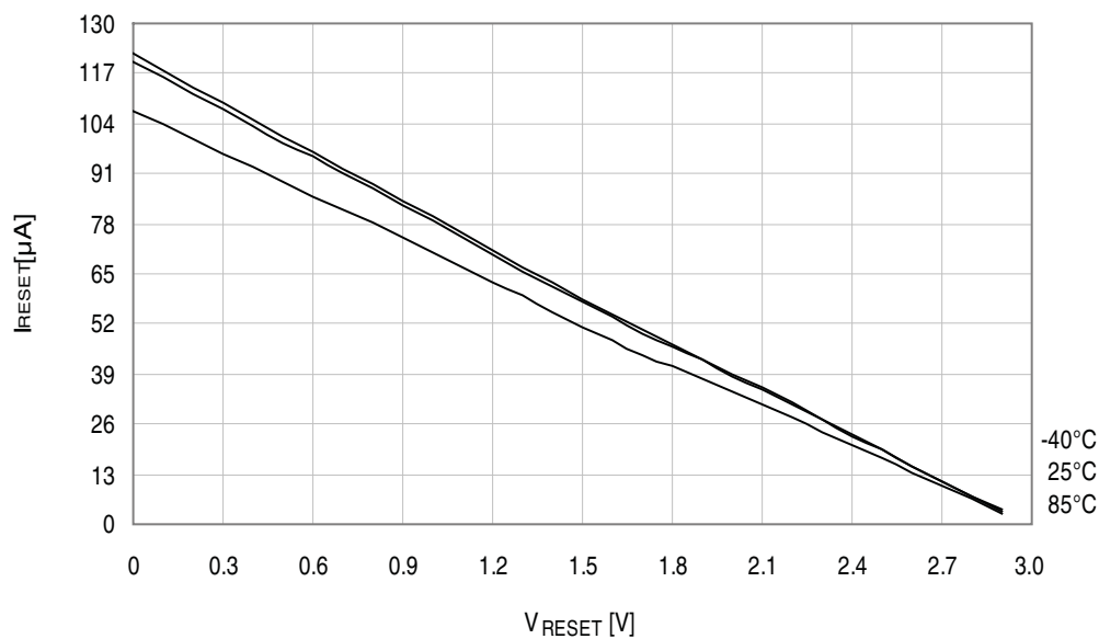
Figure 33-335. Reset pin pull-up resistor current vs. reset pin voltage. V_{CC} = 3.0V .
