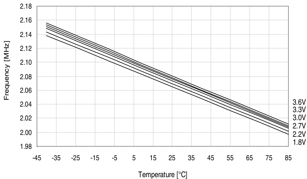
Figure 33-207. 2MHz internal oscillator frequency vs. temperature. DFLL disabled.
