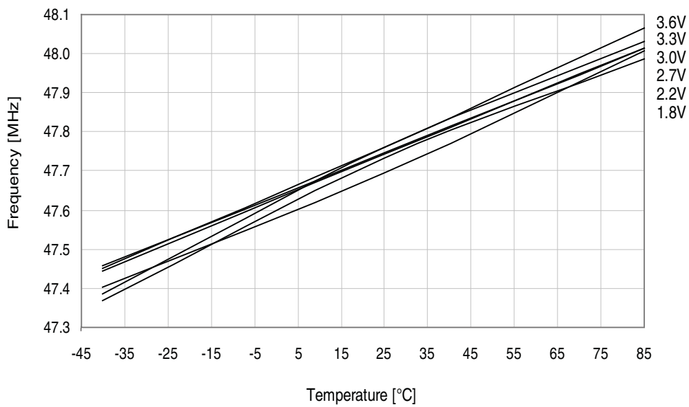
Figure 33-215. 48MHz internal oscillator frequency vs. temperature. DFLL enabled, from the 32.768kHz internal oscillator.
