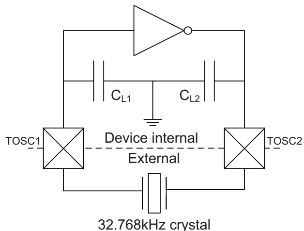
Figure 32-11.TOSC input capacitance.
