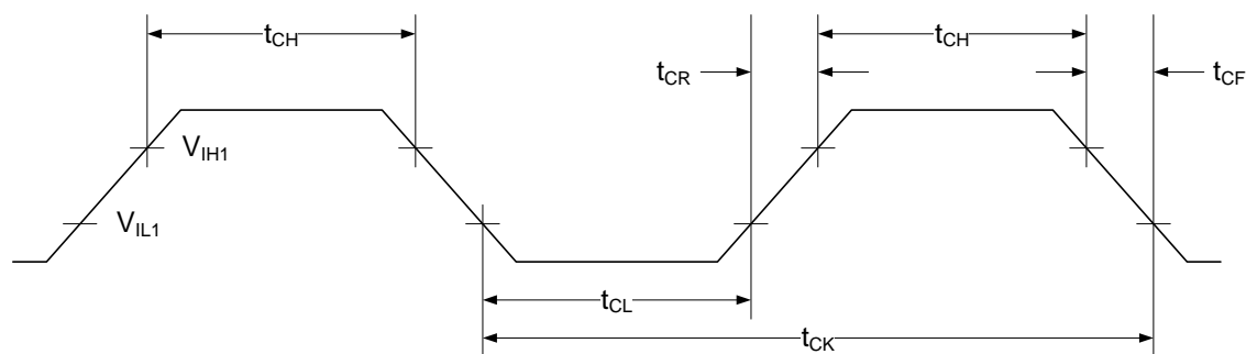
Figure 32-38. External clock drive waveform.
