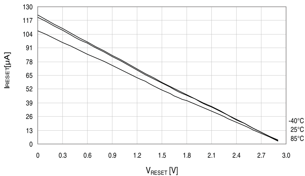
Figure 33-268. Reset pin pull-up resistor current vs. reset pin voltage. V_{CC} = 3.0V .
