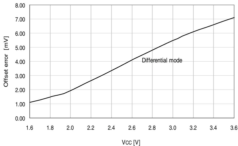
Figure 33-325. Offset error vs. V_{CC} . T = 25^{\circ}C , V_{REF} = \text{external } 1.0V , ADC sample rate = 300kps.
