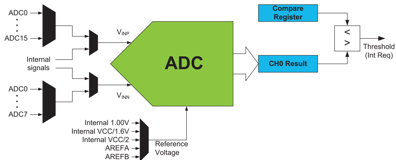
Figure 25-1. ADC overview.
