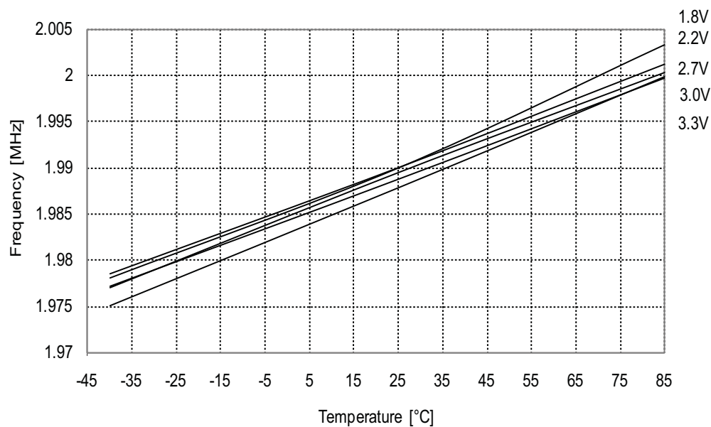
Figure 33-141. 2MHz internal oscillator frequency vs. temperature. DFLL enabled, from the 32.678kHz internal oscillator.
