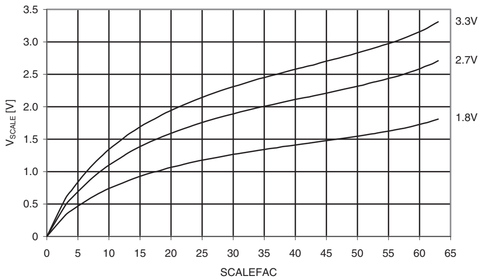
Figure 34-6. Analog comparator voltage scaler vs. scalefac.
