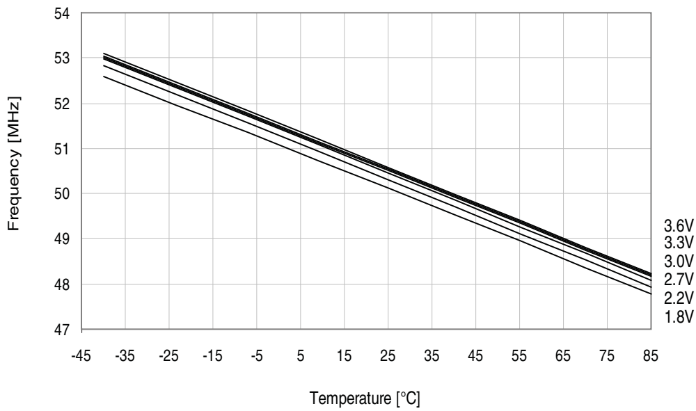
Figure 33-214. 48MHz internal oscillator frequency vs. temperature. DFLL disabled.
