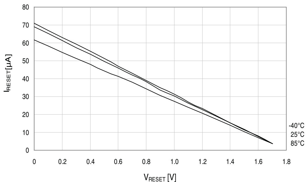
Figure 33-267. Reset pin pull-up resistor current vs. reset pin voltage. V_{CC} = 1.8V .
