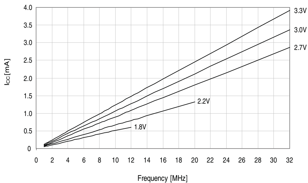
Figure 33-161. Idle mode supply current vs. V_{\text{CC}} .
