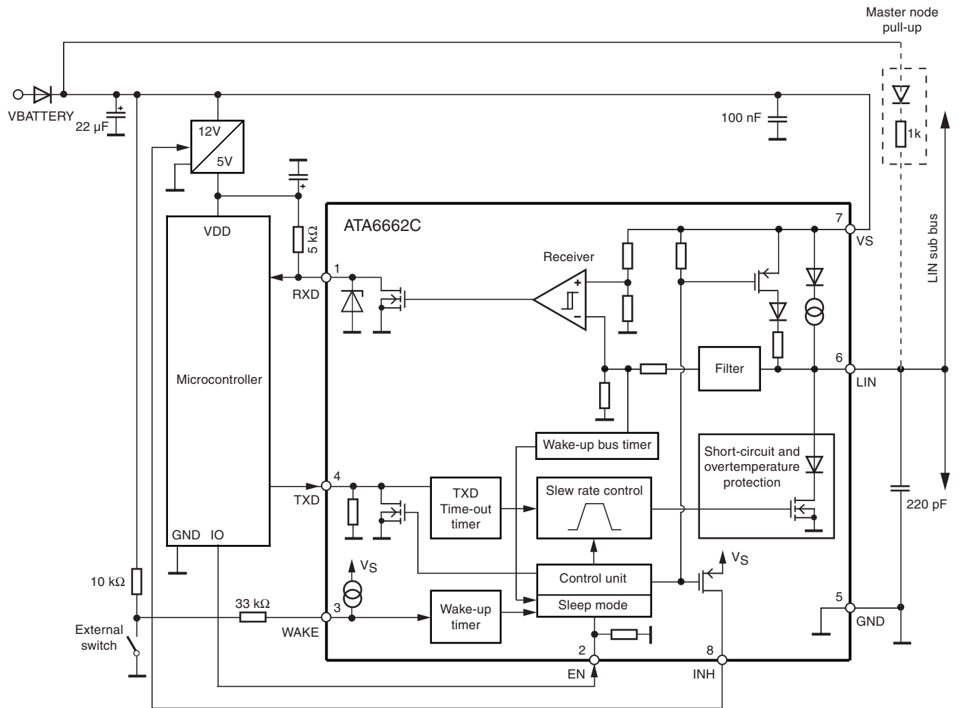
Figure 6-2. Application Circuit
