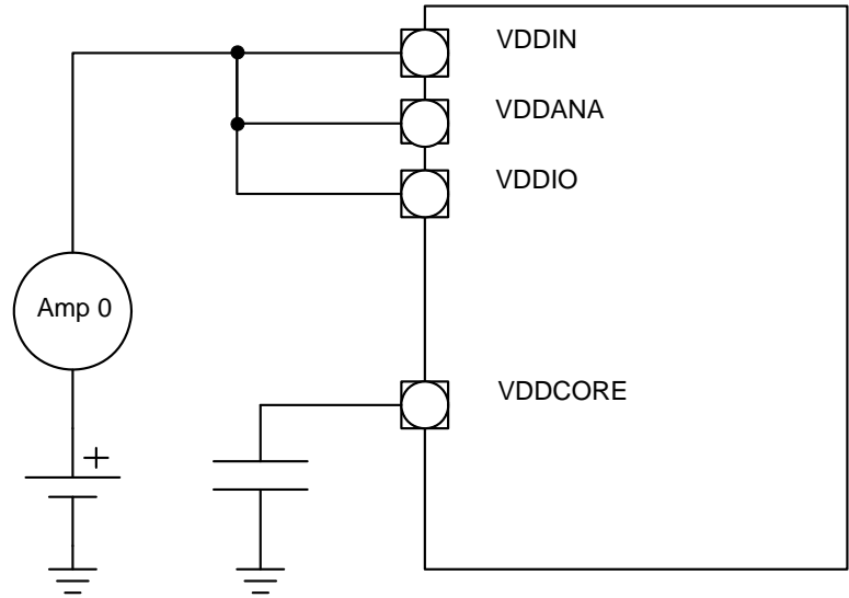
Figure 32-1. Measurement Schematic
