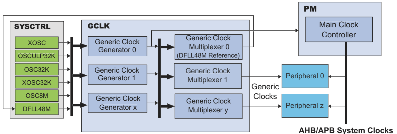
Figure 13-1. Clock distribution
