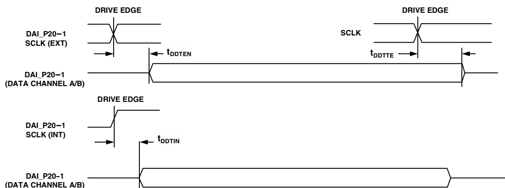
Figure 23. Serial Ports
