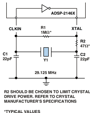
Figure 6. 450 MHz Operation (Fundamental Mode Crystal)
