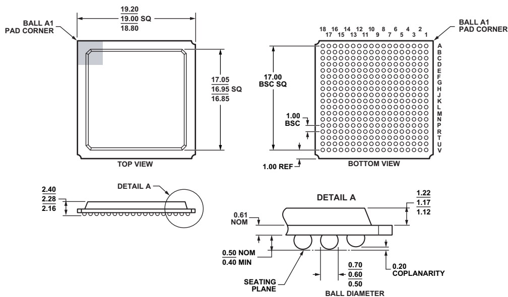
Figure 47. 324-Ball Plastic Ball Grid Array [PBGA] (B-324)
