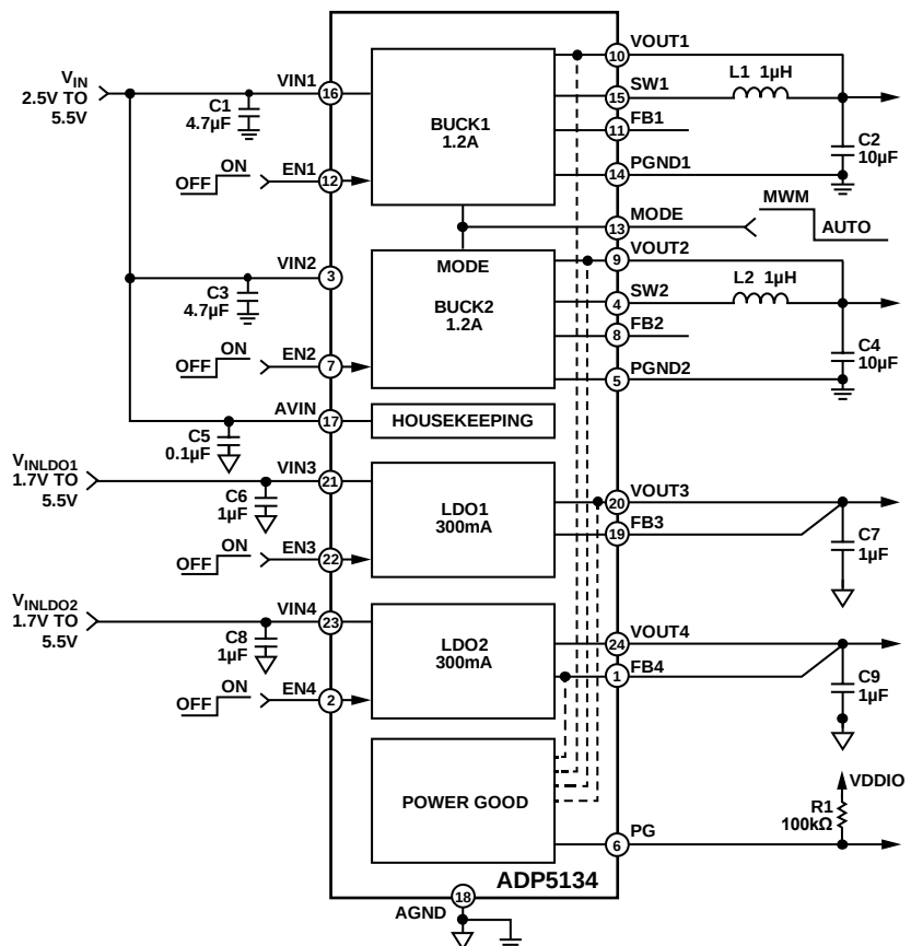
Figure 52. ADP5134 Fixed Output Voltages with Enable Pins
