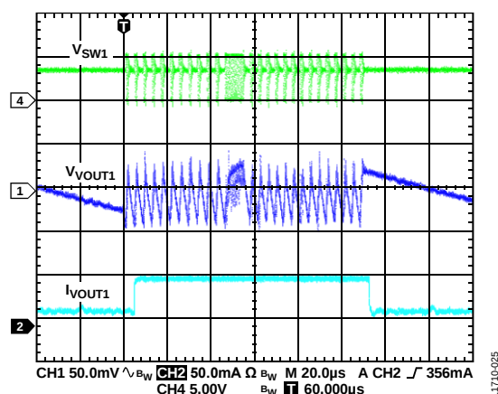
Figure 25. BUCK1 Response to Load Transient, I_{OUT1} from 1 mA to 50 mA, V_{OUT1} = 3.3\text{ V} , Auto Mode
