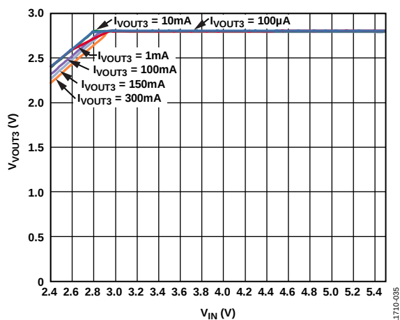
Figure 35. LDO Line Regulation Across Output Load, V_{OUT3} = 2.8\text{ V}
