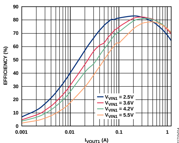
Figure 14. BUCK1 Efficiency vs. Load Current, Across Input Voltage, V_{OUT1} = 0.8\text{ V} , PWM Mode
