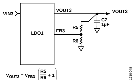
Figure 48. LDO1 External Output Voltage Setting
