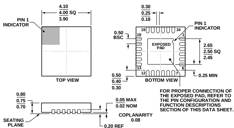
Figure 54. 24-Lead Lead Frame Chip Scale Package [LFCSP_WQ] 4 mm × 4 mm Body, Very Very Thin Quad (CP-24-7) Dimensions shown in millimeters
