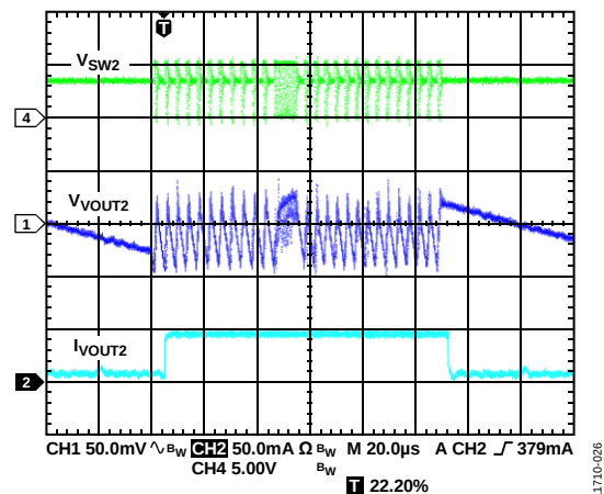
Figure 26. BUCK2 Response to Load Transient, I_{OUT2} from 1 mA to 50 mA, V_{OUT2} = 1.8\text{ V} , Auto Mode
