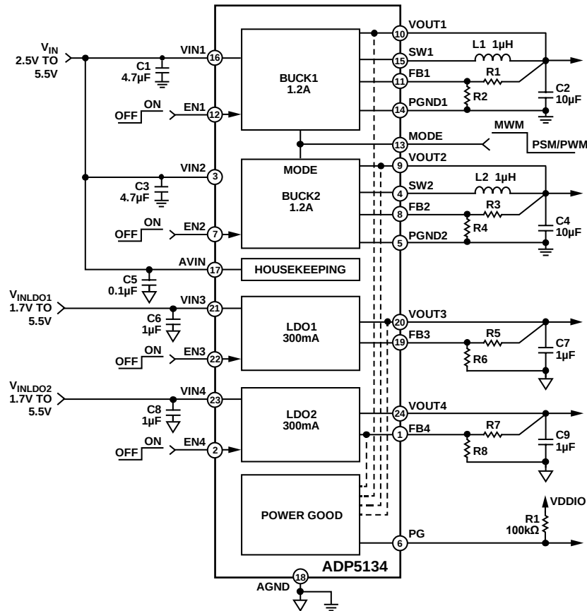
Figure 53. ADP5134 Adjustable Output Voltages with Enable Pins
