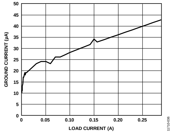
Figure 36. LDO Ground Current vs. Load Current, V_{IN3} = 3.3\text{ V} , V_{OUT3} = 2.8\text{ V}
