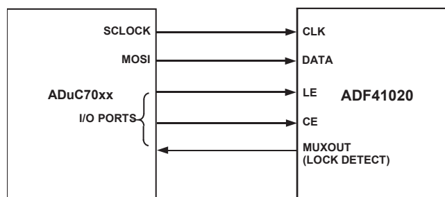
Figure 18. ADuC70xx-to-ADF41020 Interface
