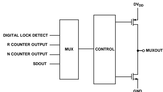
Figure 12. MUXOUT Circuit
