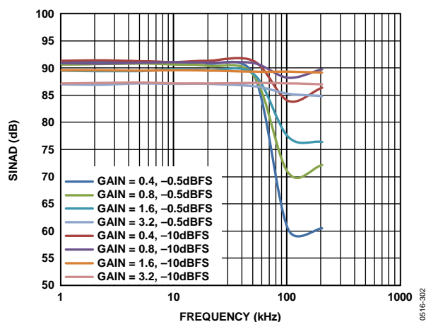
Figure 26. SINAD vs. Frequency
