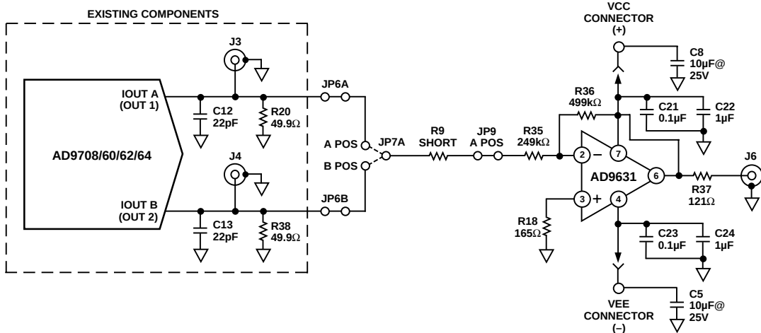
Figure 6. Inverting Amplifier Configuration
