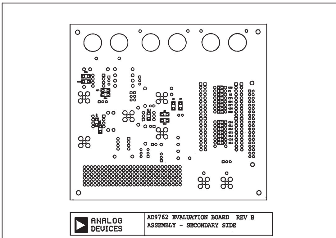
Figure 19. Silkscreen Layer—Bottom
