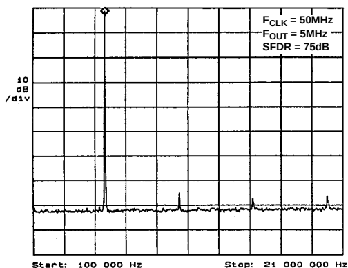
Figure 7. Resistive Output Load
