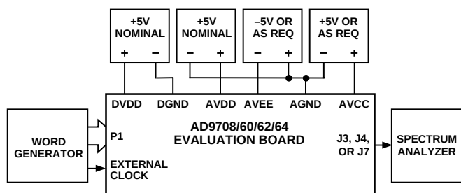
Figure 3. Equipment Setup
