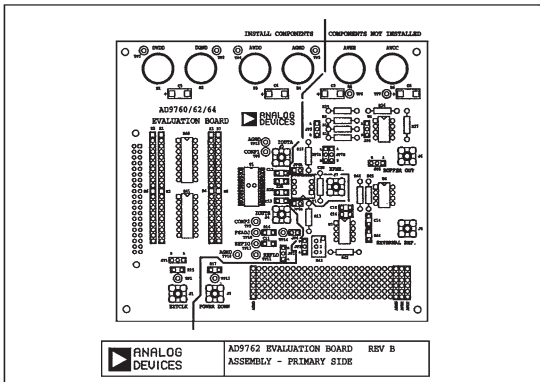
Figure 14. Silkscreen Layer—Top
