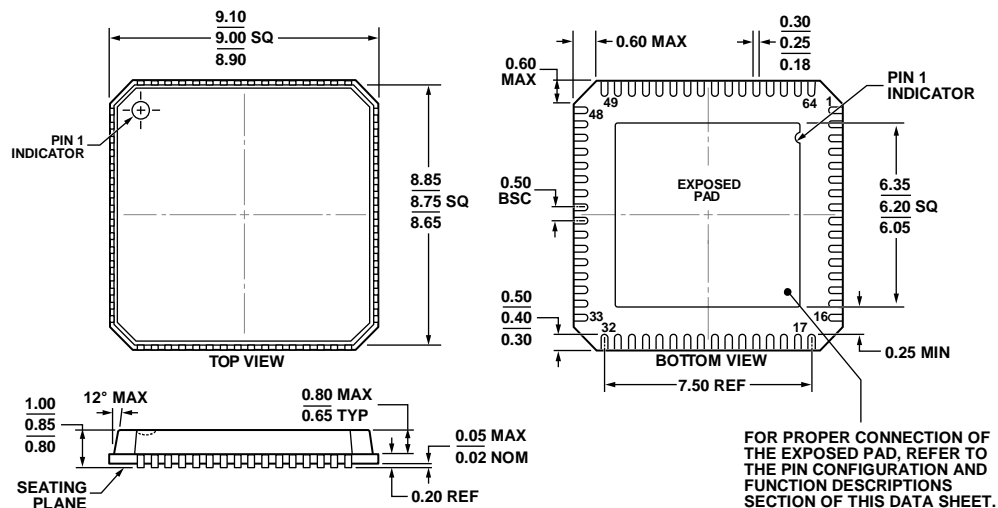
COMPLIANT TO JEDEC STANDARDS MO-220-VMMD-4 Figure 59. 64-Lead Lead Frame Chip Scale Package [LFCSP_VQ] 9 mm × 9 mm Body, Very Thin Quad (CP-64-4) Dimensions shown in millimeters
