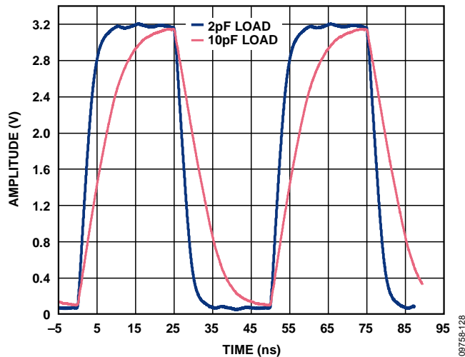
Figure 27. Output Waveform, 3.3 V CMOS (20 MHz, Weak Mode)
