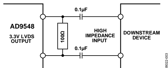
Figure 28. AC-Coupled LVDS or LVPECL Output Driver
