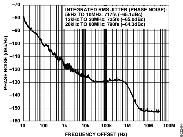
Figure 8. Additive Phase Noise (Output Driver = LVPECL), f_R = 1 Hz, f_O = 122.88 MHz, LBW = 0.05 Hz, f_{SYS} = 20 MHz (OCXO), PLL On
