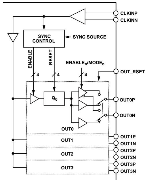
Figure 48. Clock Distribution
