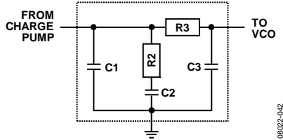
Figure 68. Third Order Analog Loop Filter
