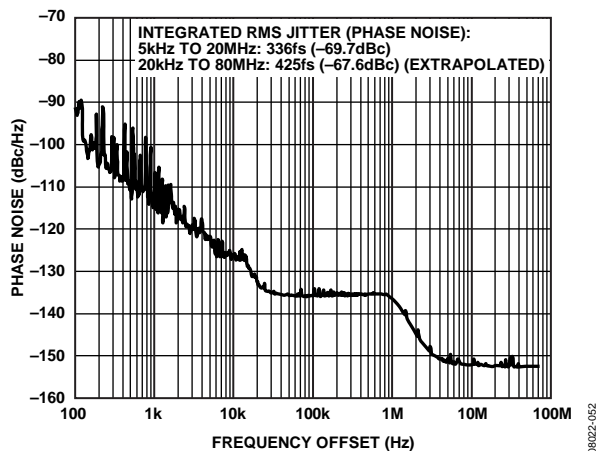
Figure 9. Additive Phase Noise (Output Driver = LVPECL), f_R = 8 kHz, f_O = 155.52 MHz, LBW = 100 Hz, f_{SYS} = 50 MHz (Crystal), PLL On
