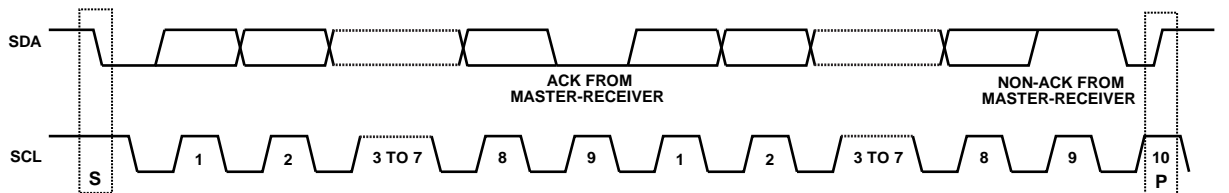
Figure 65. Data Transfer Process (Master Read Mode, 2-Byte Transfer)
