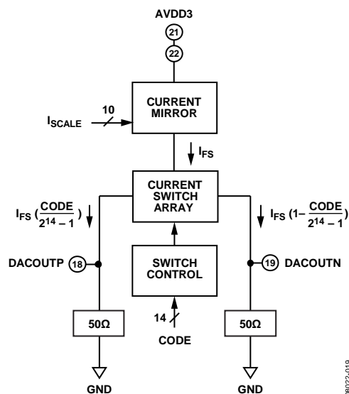
Figure 44. DAC Output Pins
