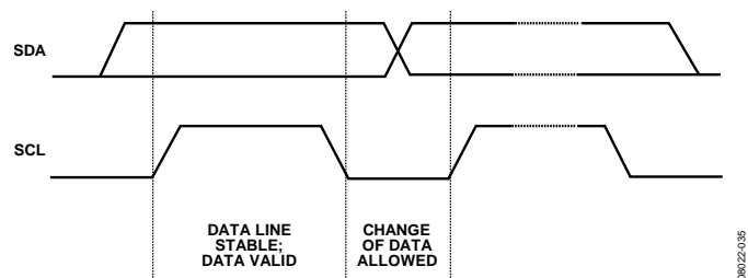
Figure 61. Valid Bit Transfer
