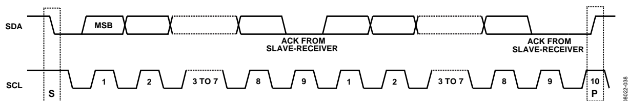
Figure 64. Data Transfer Process (Master Write Mode, 2-Byte Transfer)
