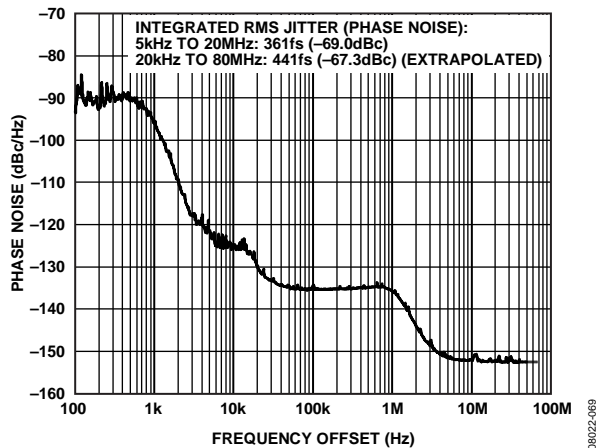
Figure 7. Additive Phase Noise (Output Driver = LVPECL), f_R = 19.44 MHz, f_O = 155.52 MHz, LBW = 1 kHz, f_{SYS} = 50 MHz, PLL On
