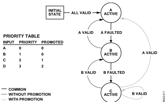
Figure 36. Example of Priority Promotion
