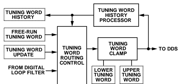
Figure 45. Tuning Word Processing
