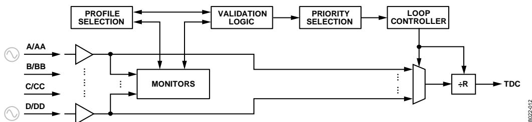
Figure 37. Reference Clock Block Diagram
