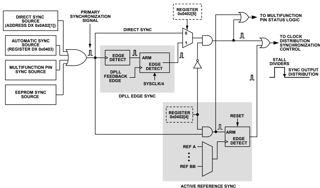
Figure 47. Output Synchronization Block Diagram
