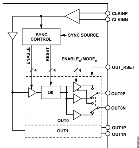
Figure 46. Clock Distribution
