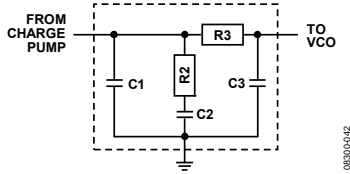
Figure 66. Third-Order Analog Loop Filter
