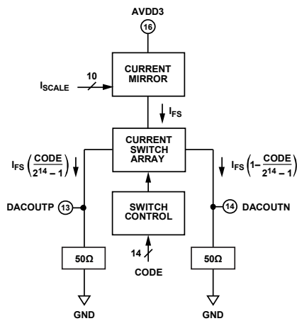
Figure 42. DAC Output Pins
