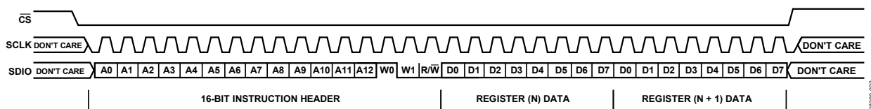
Figure 57. Serial Control Port Write—LSB First, 16-Bit Instruction, Two Bytes of Data
