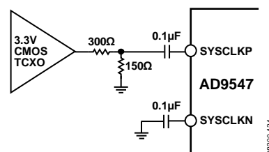
Figure 31. System Clock Input (SYSCLKP/SYSCLKN) When Using a TCXO/OCXO with 3.3 V CMOS Output
