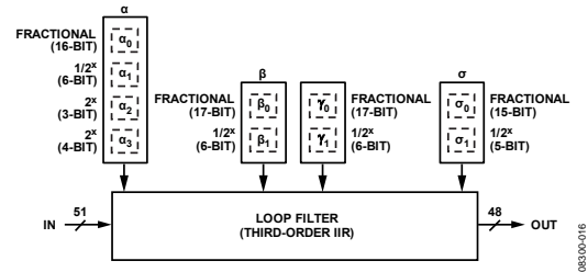
Figure 39. Third-Order Digital IIR Loop Filter
