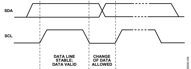
Figure 59. Valid Bit Transfer
