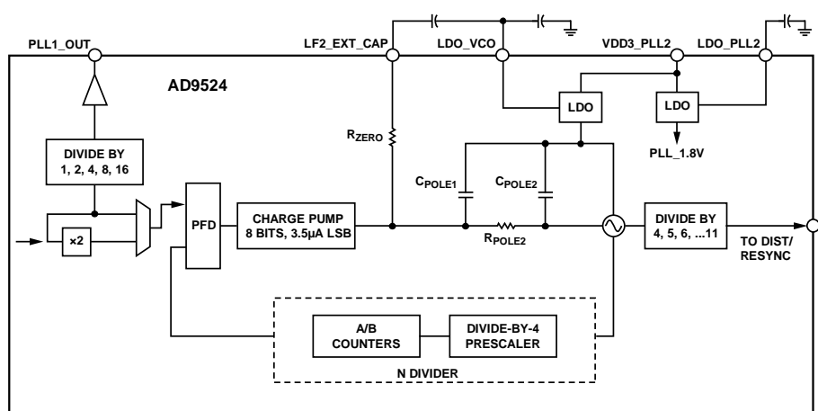
Figure 25. Output PLL (PLL2) Block Diagram
