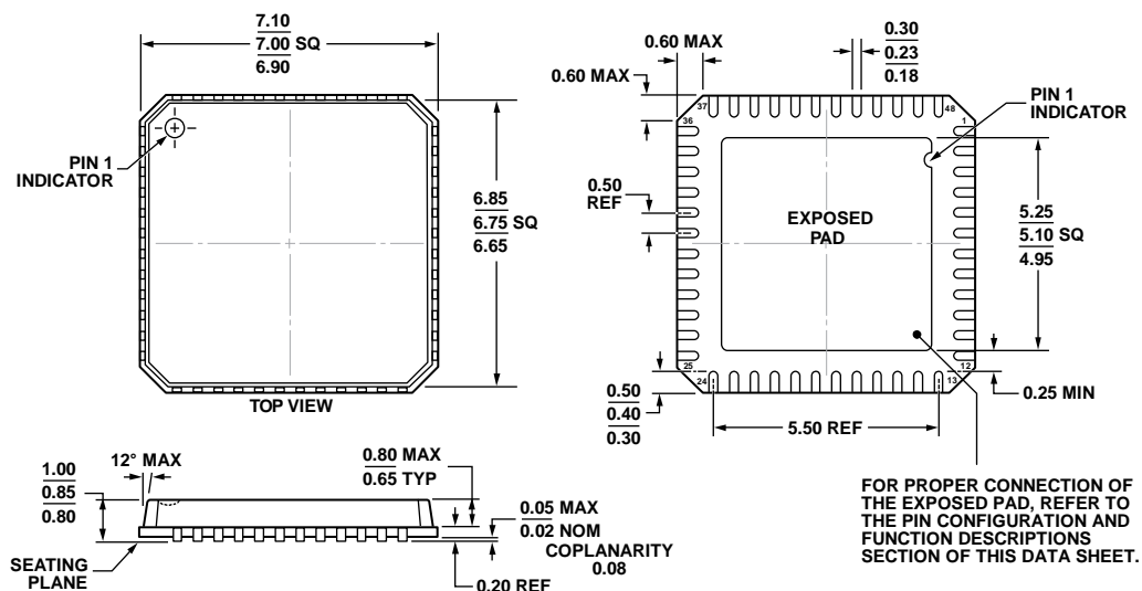
Figure 45. 48-Lead Lead Frame Chip Scale Package [LFCSP_VQ]
