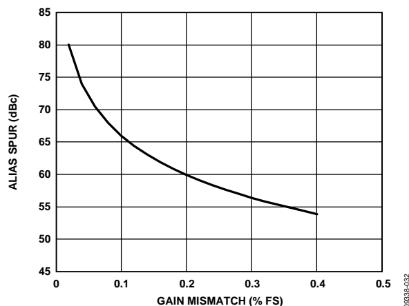
Figure 30. AS_{\text{GAIN}} as a Function of Gain Mismatch
