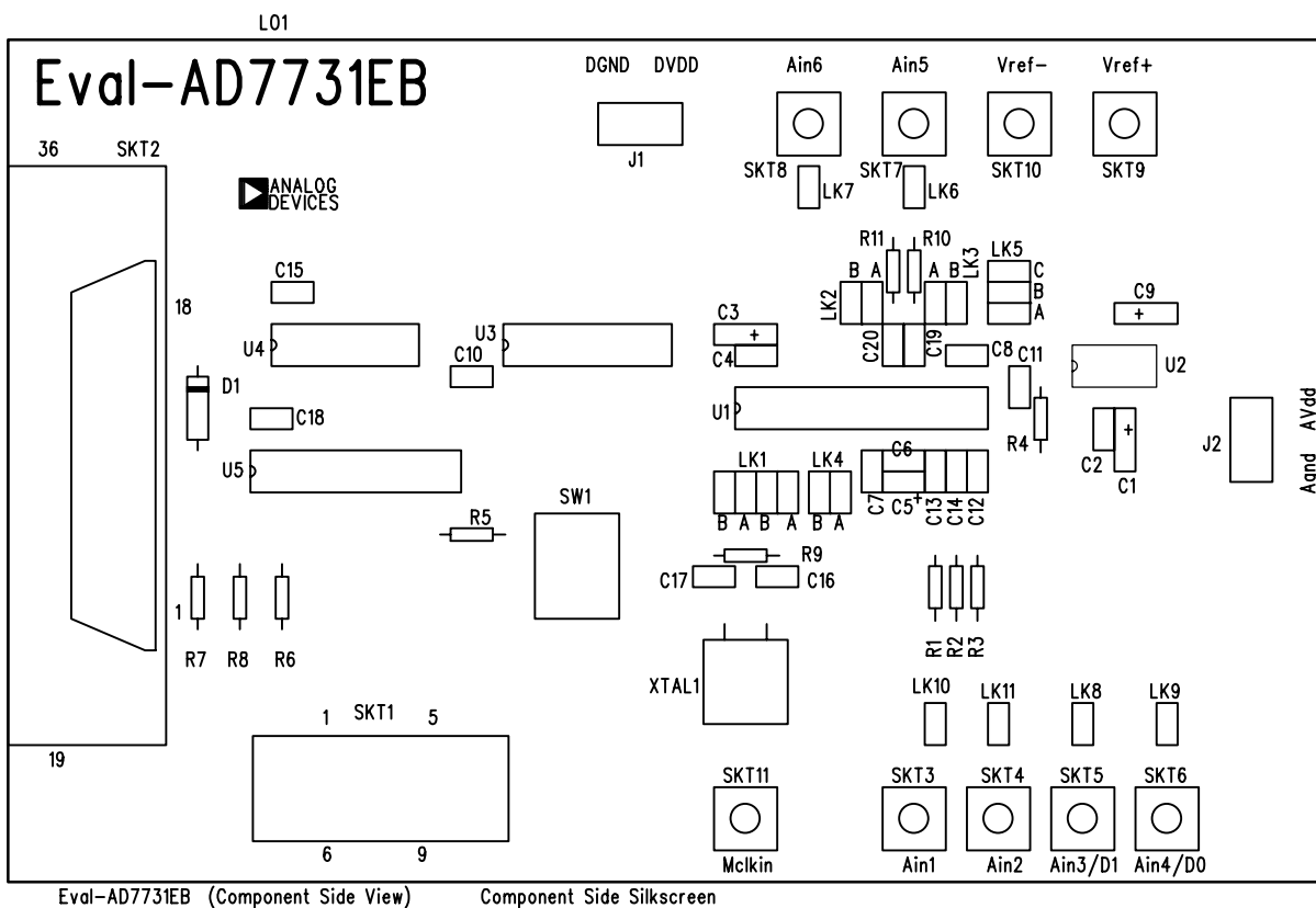
Figure 3. Eval-AD7731EB Silkscreen Artwork.
