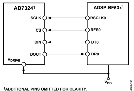
Figure 53. Interfacing the AD7324 to the ADSP-BF53x
