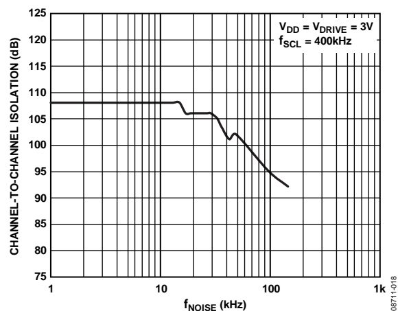
Figure 13. Channel-to-Channel Isolation, f_{IN} = 10 kHz
