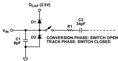
Figure 20. Equivalent Analog Input Circuit
