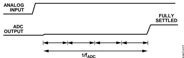
Figure 31. \text{Sinc}^4 Zero Latency Operation
