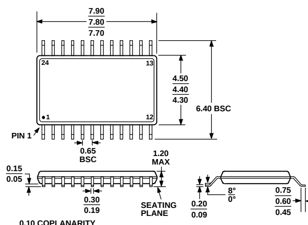
Figure 33. 24-Lead Thin Shrink Small Outline Package [TSSOP] (RU-24) Dimensions shown in millimeters
