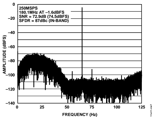
Figure 47. 22% Bandwidth Mode, Tuning Word = 41
