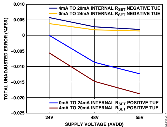
Figure 12. Total Unadjusted Error Current Mode, Internal R_{SET} Sense Resistor
