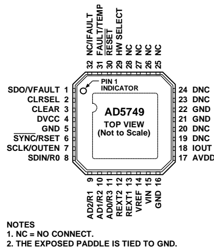
Figure 4. Pin Configuration
