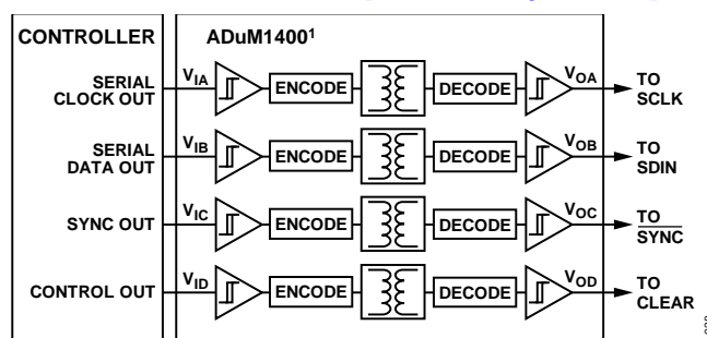
Figure 37. Isolated Interface
