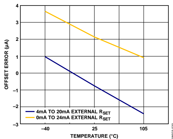
Figure 20. Offset Error vs. Temperature, External R_{SET} Sense Resistor
