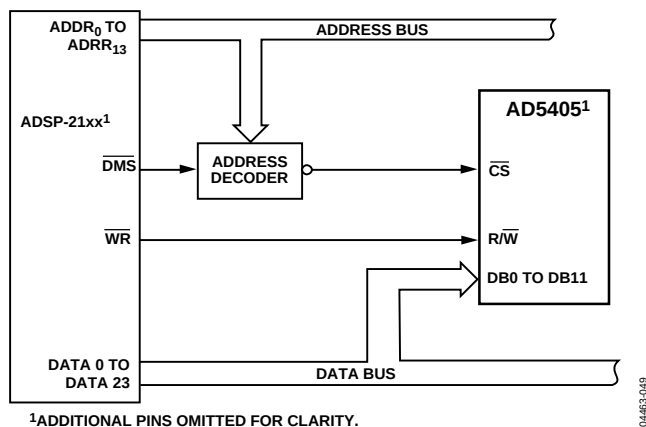
Figure 38. ADSP21xx-to-AD5405 Interface
