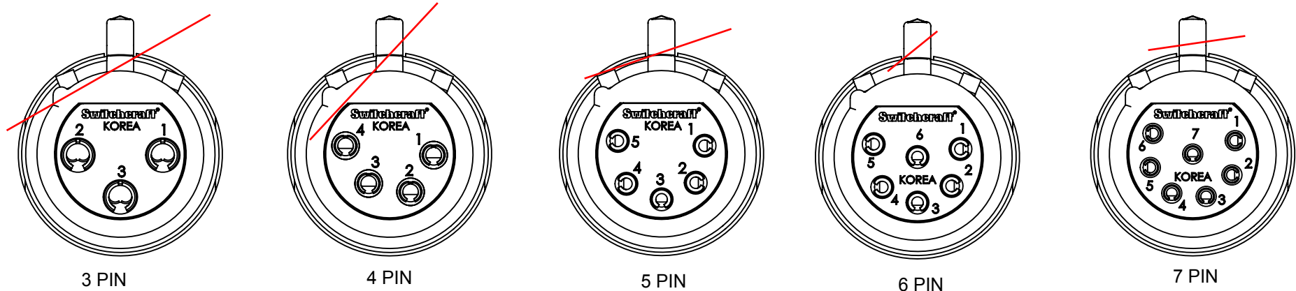
CONTACT ARRANGEMENT (SHOWN FACING THE CONNECTORS)
