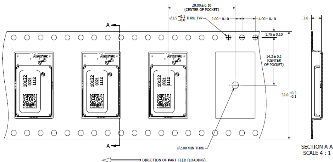
Figure 11 A2530R24A00GR and A2530R24C00GR Tape-Reel Packaging Detail (500/Reel)
