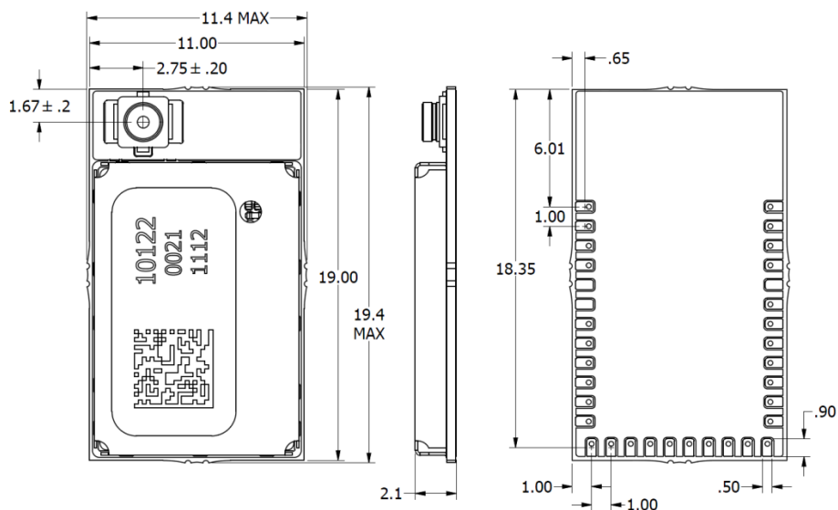
Figure 9 A2530R24C dimensions
