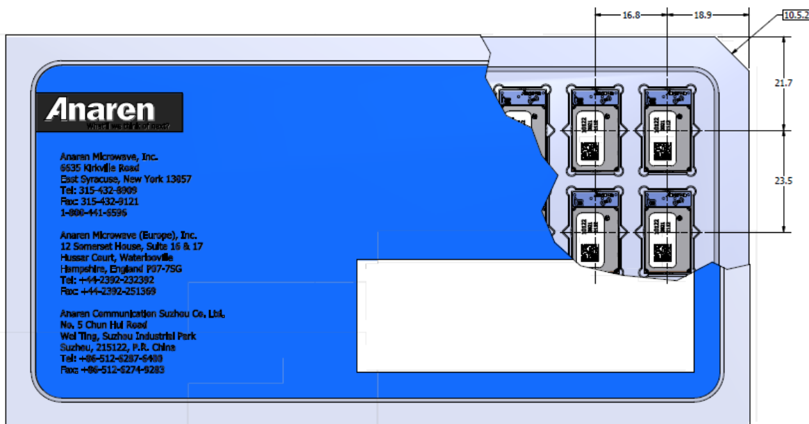
Figure 10 A2530R24A00GM and A2530R24C00GM Matrix Tray Packaging Detail (27/Tray)
