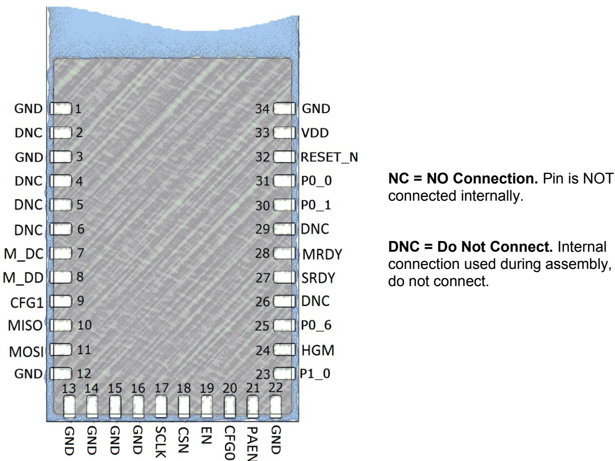
Figure 4 Module pin-out view
