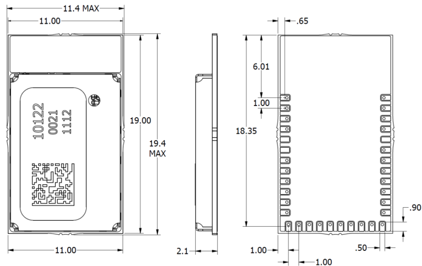
Figure 8 A2530E24A dimensions
