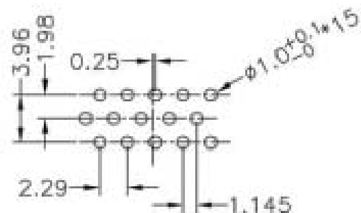
15 Pin Male Connector PCB Pin Layout Scale 2:1
